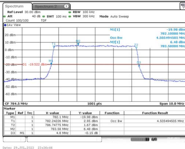
Band13-5MHz-QPSK-23255-25RB#0-4.505
