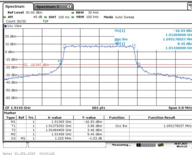
Band25-1.4MHz-QPSK-26683-6RB#0-1.093
