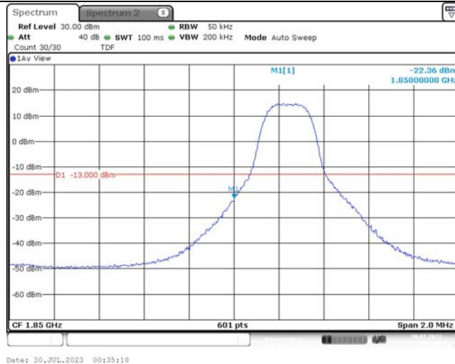
Band25-3MHz-16QAM-26055-1RB#14
