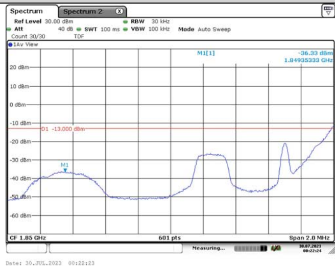
Band25-1.4MHz-QPSK-26047-6RB#0
