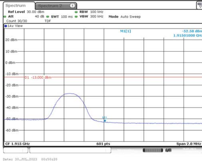
Band25-5MHz-16QAM-26665-1RB#24
