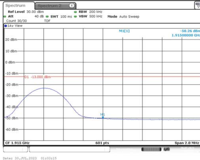
Band25-10MHz-QPSK-26640-1RB#49
