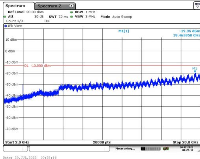
Band25-1.4MHz-QPSK-26047-1RB#0-Range3:2000~20000MHz
