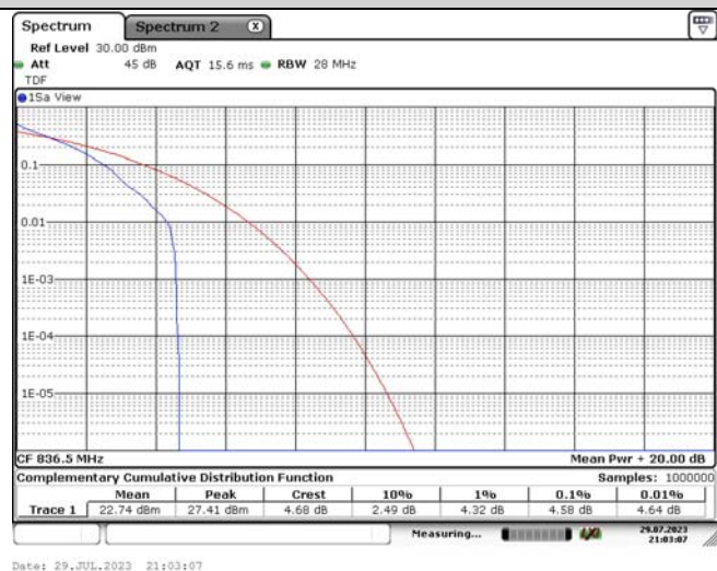
Band5-1.4MHz-QPSK-20525-1RB#0
