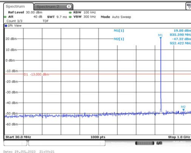
Band5-1.4MHz-QPSK-20525-1RB#0-Range1:30~1000MHz
