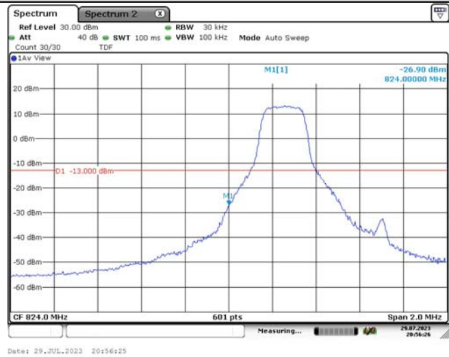
Band5-1.4MHz-QPSK-20407-1RB#5
