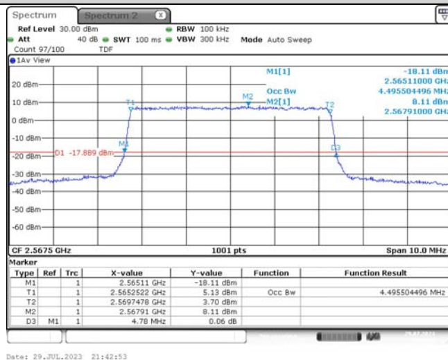
Band7-5MHz-QPSK-21425-25RB#0-4.496
