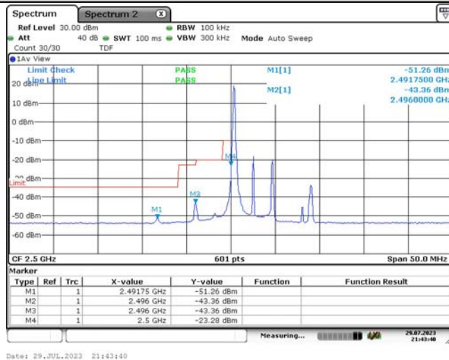
Band7-5MHz-QPSK-20775-1RB#24
