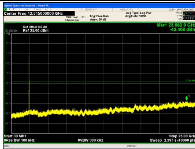
802.11g_2462_0~Reference
