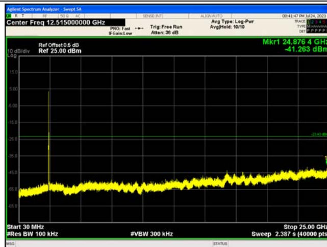
802.11n(HT20)_2462_0~Reference
