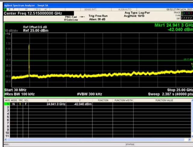
802.11n(HT40)_2437_0~Reference
