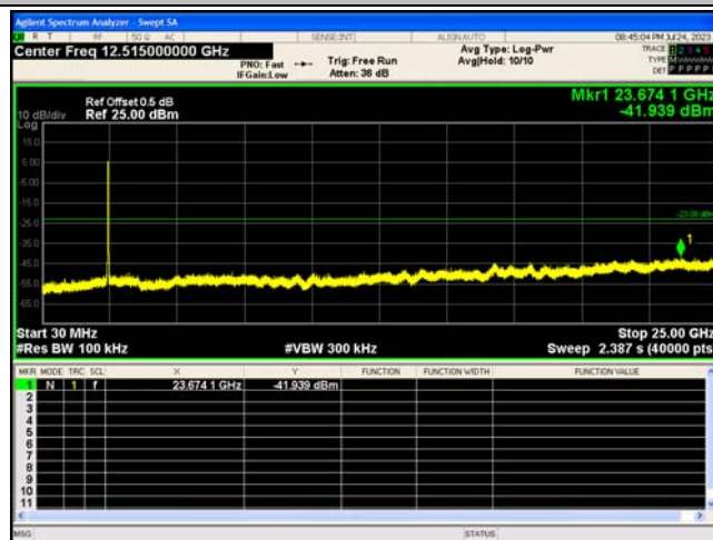
802.11n(HT40)_2422_0~Reference
