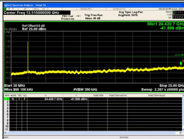
802.11n(HT20)_2412_0~Reference
