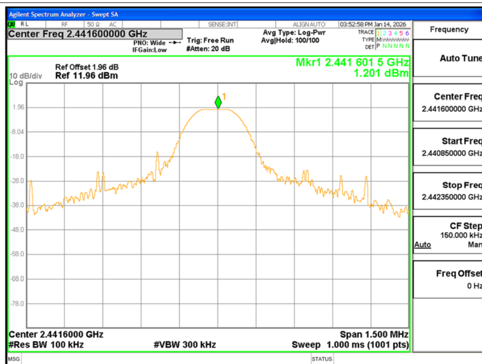
Tx. Spurious NVNT GFSK 2441.6MHz Ant1 Emission
