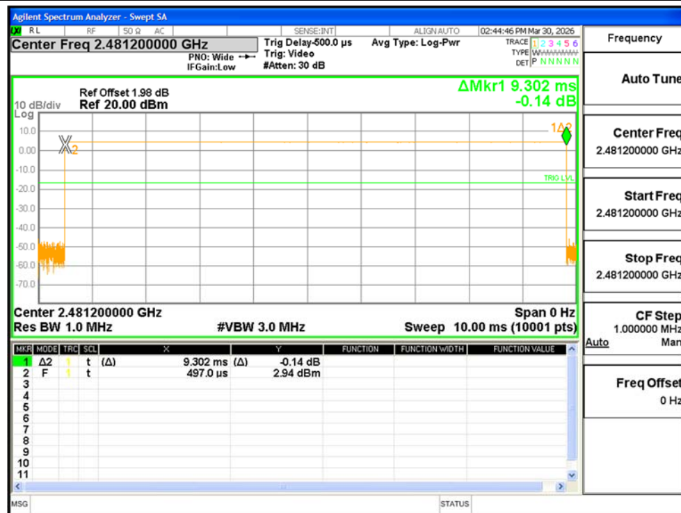
Dwell NVNT GFSK 2481.2MHz Ant1 Accumulated
