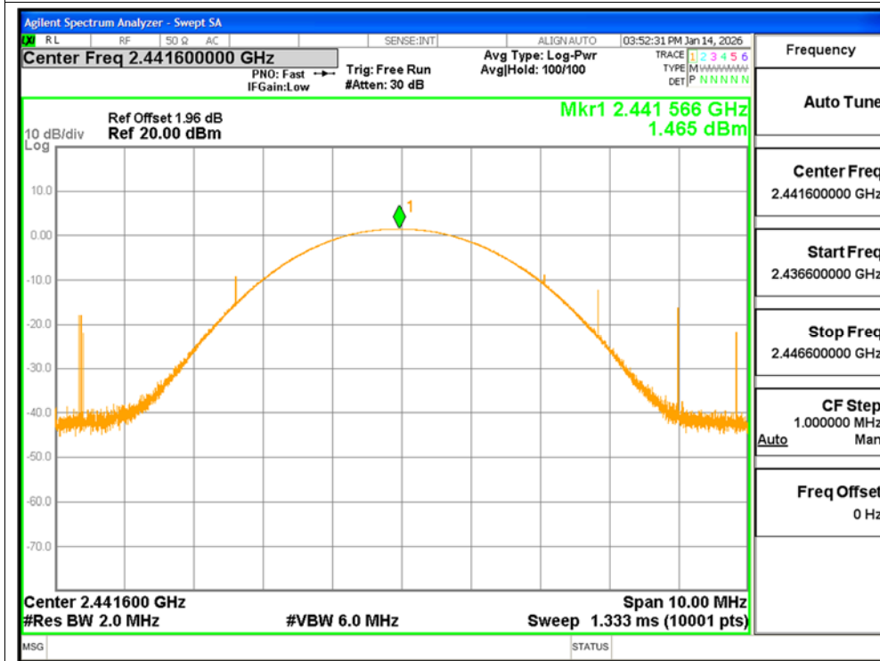
Power NVNT GFSK 2441.6MHz Ant1
