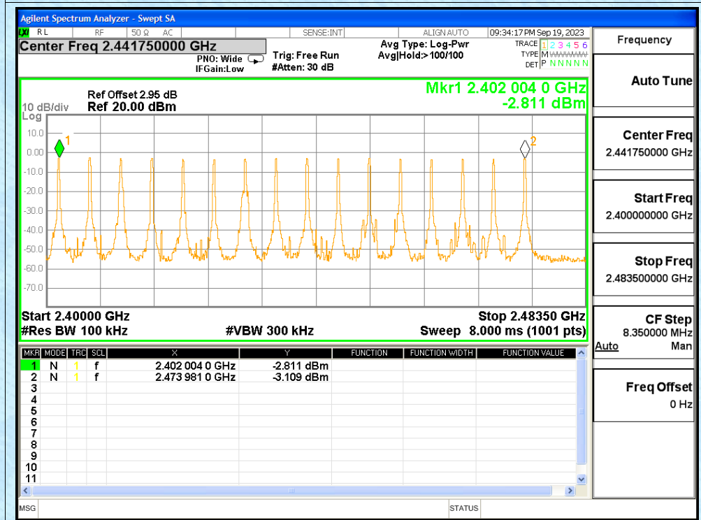
Hopping No. NVNT GFSK 2435.6MHz Ant1
