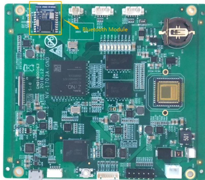
PCB
