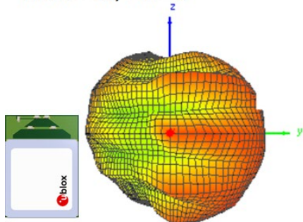
Theta = 90, Phi = 0
