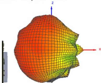
Theta = 90, Phi = 270
