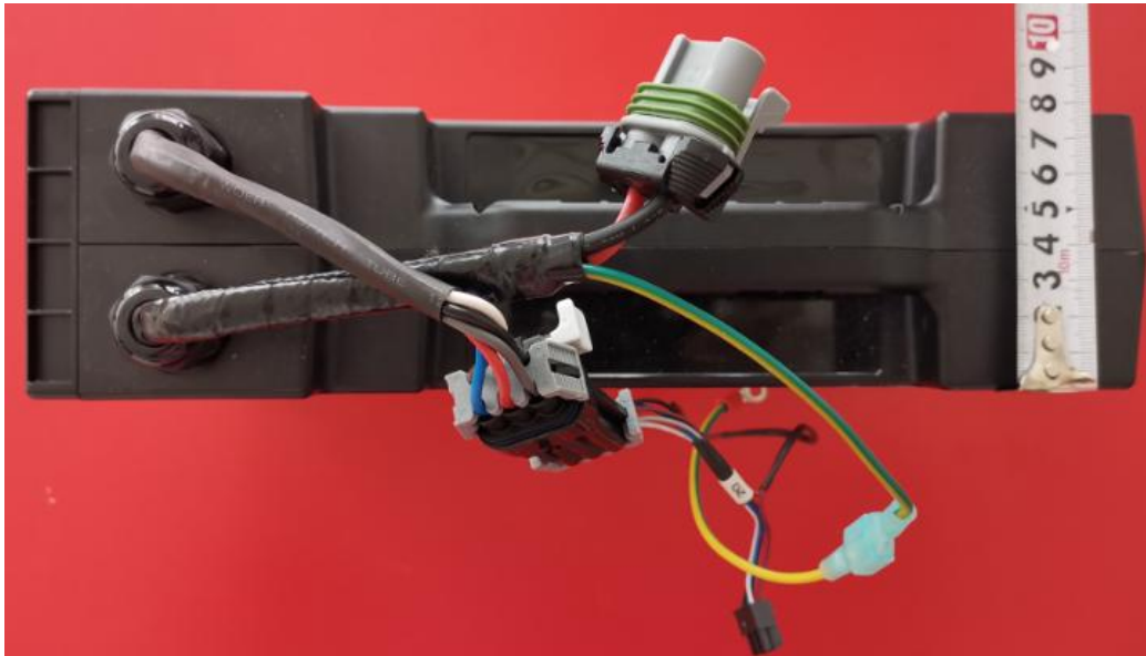
The battery view (TOCAD ENERGY Co., Ltd.)
