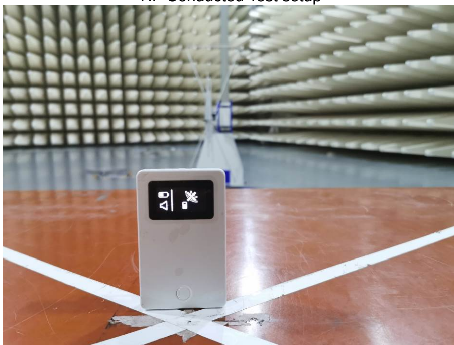
Spurious Radiated Emissions Test setup (Transmitter)
