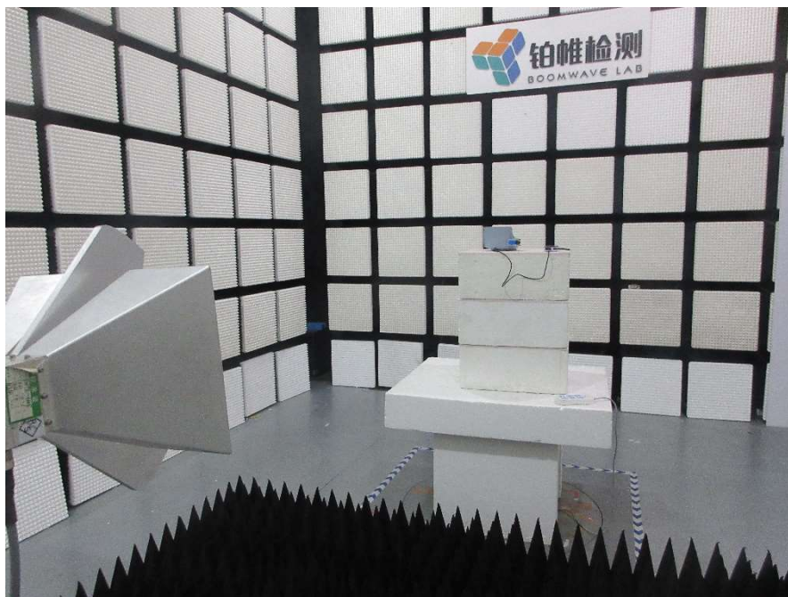
Radiated Emission 1GHz-6GHz (Rear view) – Mode 1
