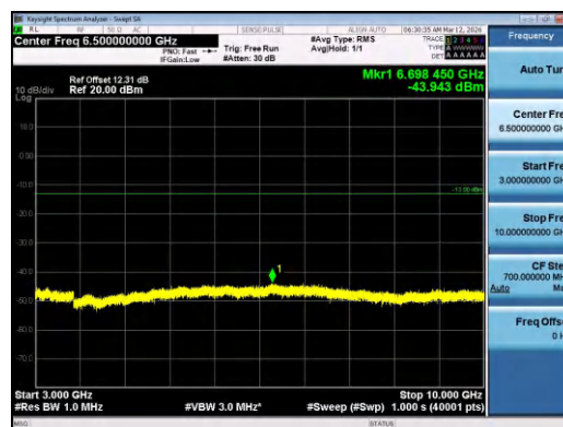
Band12-3MHz-QPSK-23165-1RB#14-3000~10000-PASS
