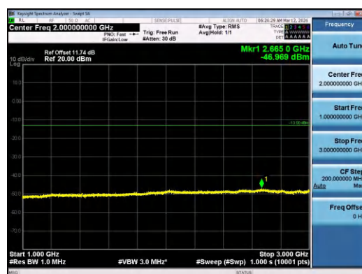
Band12-3MHz-QPSK-23095-15RB#0-1000~3000-PAS
