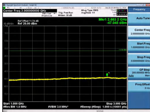
Band12-3MHz-QPSK-23165-1RB#14-1000~3000-PAS
