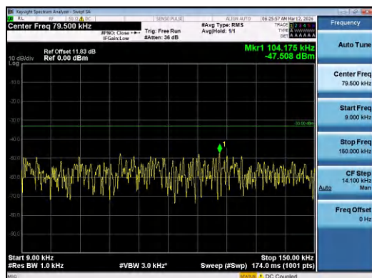
Band12-3MHz-QPSK-23095-15RB#0-0.009~0.15-PAS
