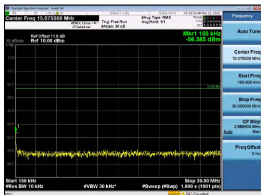
Band12-3MHz-QPSK-23165-1RB#14-0.15~30-PASS
