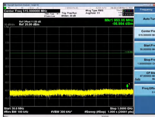
Band12-3MHz-QPSK-23165-1RB#14-30~1000-PASS
