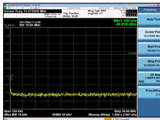
Band12-3MHz-QPSK-23095-15RB#0-0.15~30-PASS
