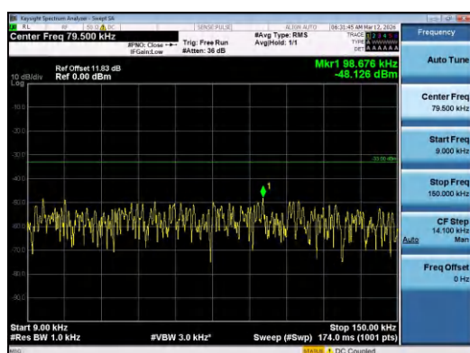
Band12-3MHz-QPSK-23165-15RB#0-0.009~0.15-PAS
