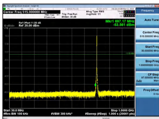
Band12-3MHz-QPSK-23095-15RB#0-30~1000-PASS
