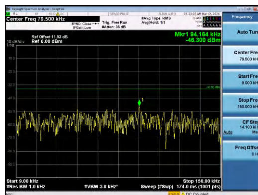
Band12-3MHz-16QAM-23095-1RB#0-0.009~0.15-PAS
