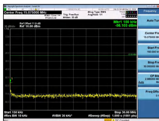
Band12-3MHz-QPSK-23165-15RB#0-0.15~30-PASS
