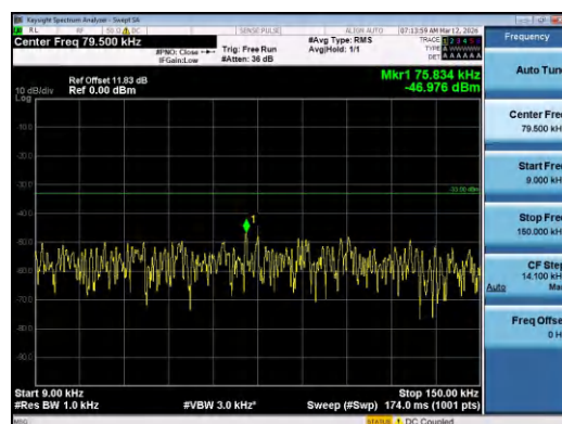
Band12-5MHz-16QAM-23095-1RB#0-0.009~0.15-PAS
