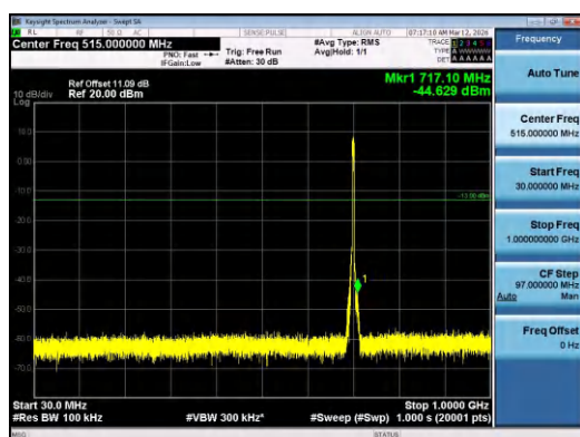
Band12-5MHz-QPSK-23095-25RB#0-30~1000-PASS
