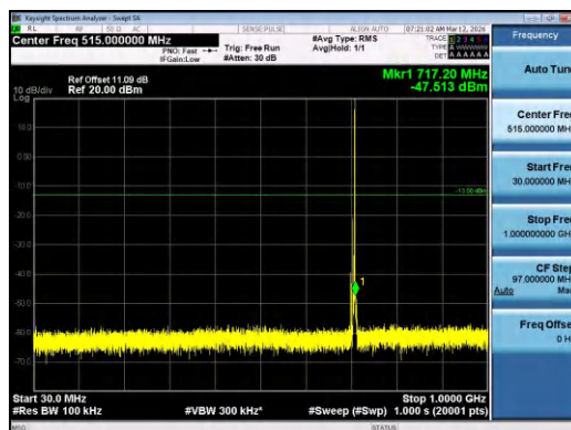
Band12-5MHz-QPSK-23155-1RB#24-30~1000-PASS
