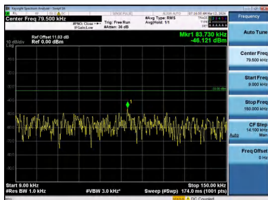
Band12-5MHz-QPSK-23095-25RB#0-0.009~0.15-PAS
