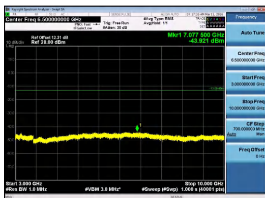
Band12-5MHz-QPSK-23095-25RB#0-3000~10000-PA
