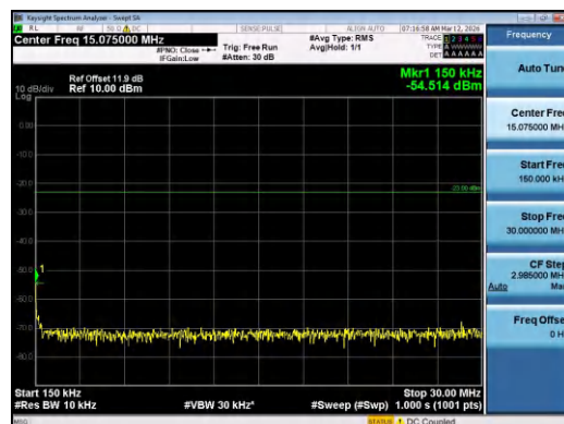
Band12-5MHz-QPSK-23095-25RB#0-0.15~30-PASS
