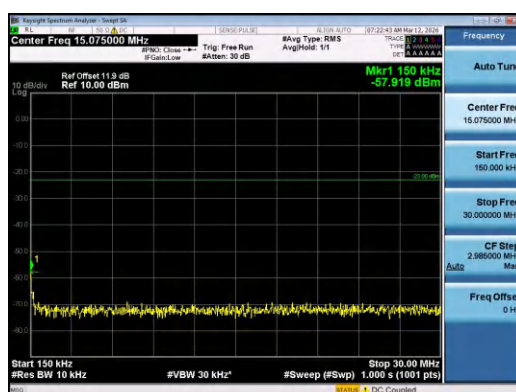
Band12-5MHz-QPSK-23155-25RB#0-0.15~30-PASS
