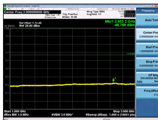
Band12-5MHz-QPSK-23095-25RB#0-1000~3000-PAS
