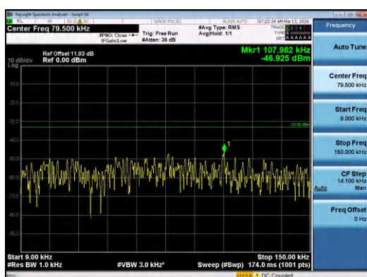
Band12-5MHz-QPSK-23155-25RB#0-0.009~0.15-PAS
