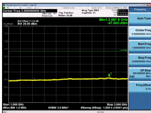
Band12-5MHz-QPSK-23155-1RB#24-1000~3000-PAS
