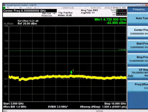
Band12-5MHz-QPSK-23155-1RB#24-3000~10000-PASS
