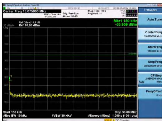
Band12-5MHz-QPSK-23155-1RB#24-0.15~30-PASS
