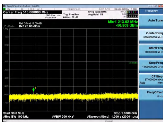
Band4-20MHz-QPSK-20175-100RB#0-30~1000-PASS
