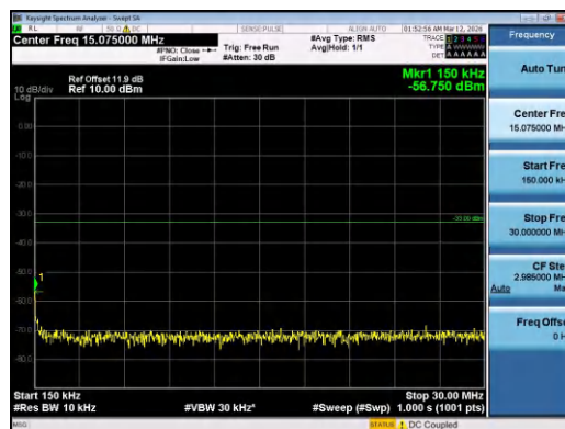
Band4-20MHz-QPSK-20175-100RB#0-0.15~30-PASS
