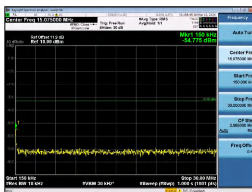
Band4-20MHz-QPSK-20300-100RB#0-0.15~30-PASS
