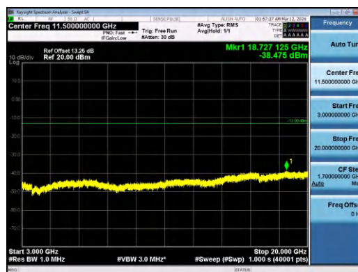
Band4-20MHz-QPSK-20300-1RB#99-3000~20000-PA
