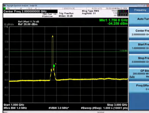
Band4-20MHz-QPSK-20175-100RB#0-1000~3000-PA
