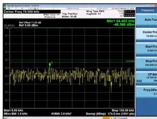
Band4-20MHz-16QAM-20175-1RB#0-0.009~0.15-PAS
