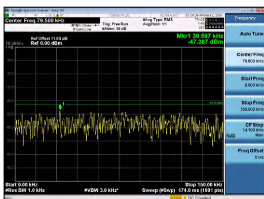
Band4-20MHz-QPSK-20300-100RB#0-0.009~0.15-PA
