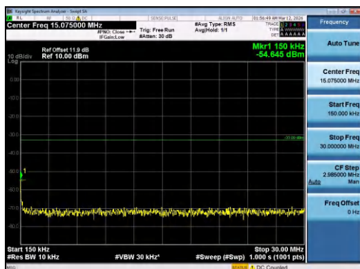
Band4-20MHz-QPSK-20300-1RB#99-0.15~30-PASS
