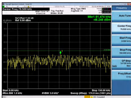
Band4-20MHz-QPSK-20175-100RB#0-0.009~0.15-PA
