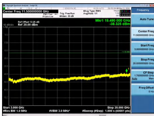
Band4-20MHz-QPSK-20175-100RB#0-3000~20000-P
