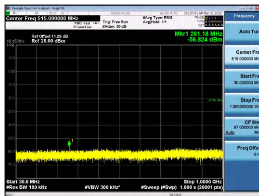
Band4-20MHz-QPSK-20300-1RB#99-30~1000-PASS
