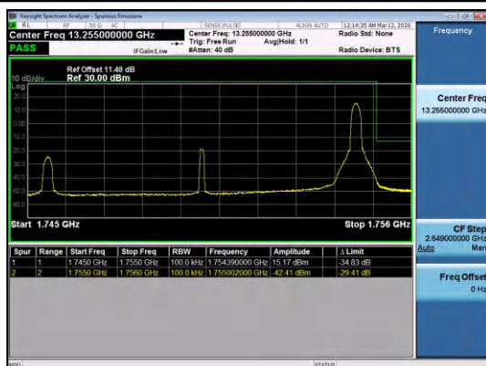
Band4-10MHz-16QAM-20350-1RB#49-PASS
