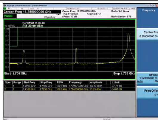
Band4-15MHz-QPSK-2025-1RB#74-PASS
