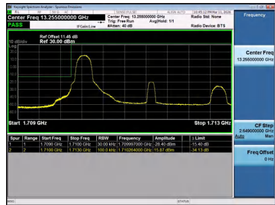
Band4-3MHz-16QAM-19965-1RB#0-PASS
