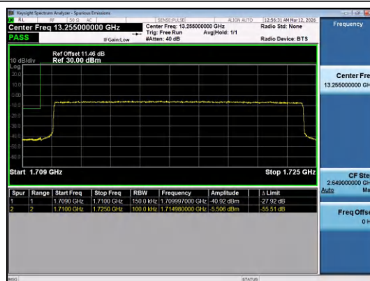
Band4-15MHz-16QAM-2025-75RB#0-PASS
