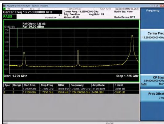
Band4-15MHz-16QAM-2025-1RB#74-PASS
