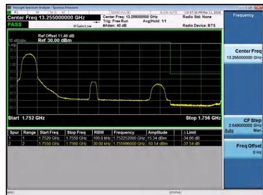
Band4-3MHz-16QAM-20385-1RB#0-PASS
