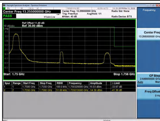
Band4-5MHz-QPSK-20375-1RB#0-PASS
