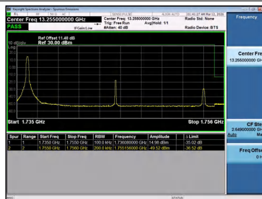
Band4-20MHz-16QAM-20300-1RB#0-PASS
