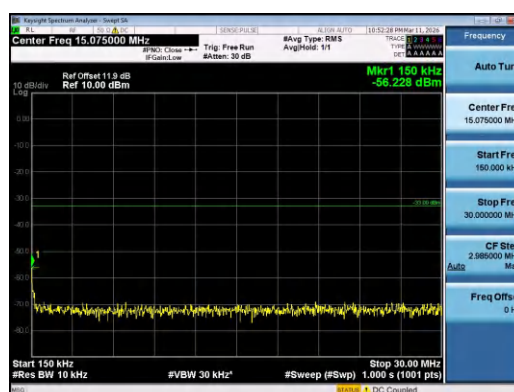
Band4-3MHz-16QAM-19965-1RB#14-0.15~30-PASS
