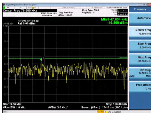
Band4-3MHz-16QAM-20175-1RB#14-0.009~0.15-PAS
