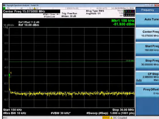
Band4-5MHz-QPSK-19975-1RB#24-0.15~30-PASS
