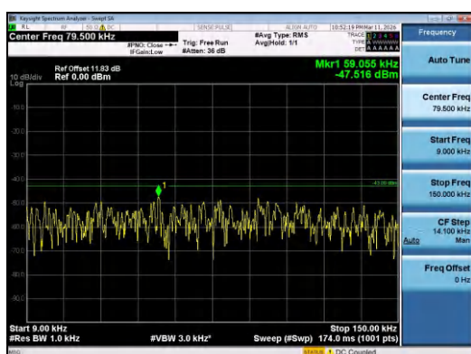
Band4-3MHz-16QAM-19965-1RB#14-0.009~0.15-PAS
