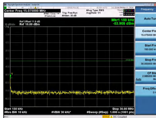
Band4-5MHz-QPSK-19975-1RB#0-0.15~30-PASS
