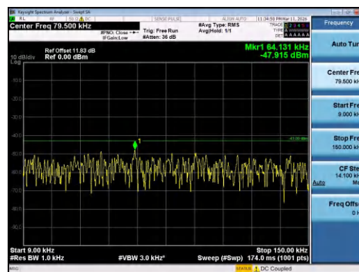
Band4-5MHz-QPSK-19975-1RB#24-0.009~0.15-PASS
