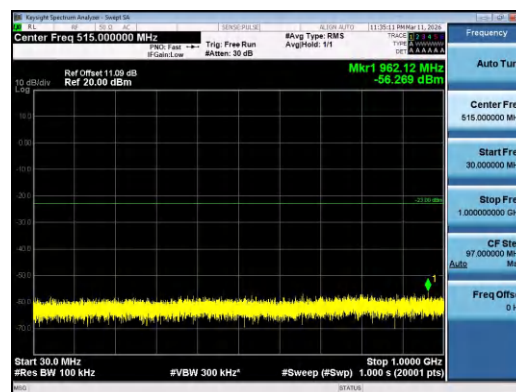
Band4-5MHz-QPSK-19975-1RB#24-30~1000-PASS
