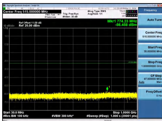
Band4-5MHz-QPSK-19975-1RB#0-30~1000-PASS
