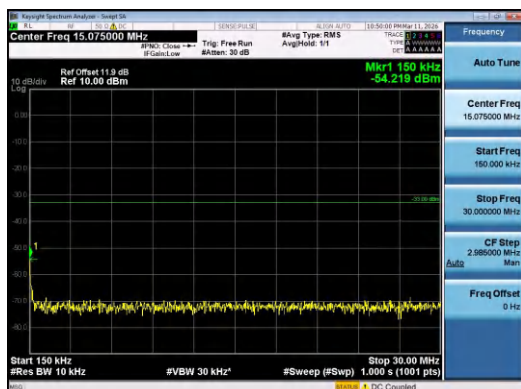
Band4-3MHz-16QAM-19965-1RB#0-0.15~30-PASS
