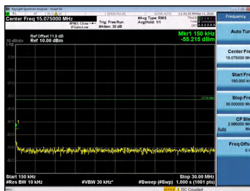
Band4-5MHz-QPSK-20175-25RB#0-0.15~30-PASS
