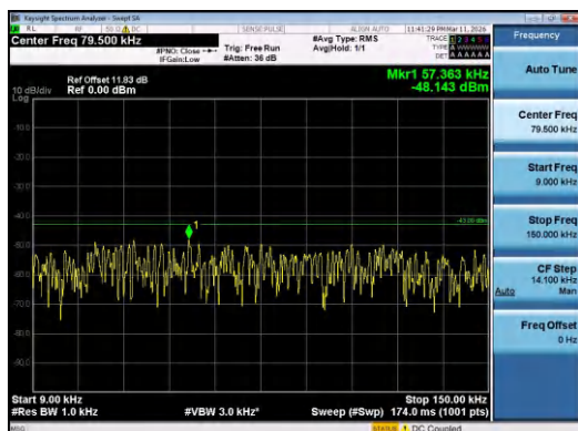
Band4-5MHz-16QAM-20175-1RB#24-0.009~0.15-PAS
