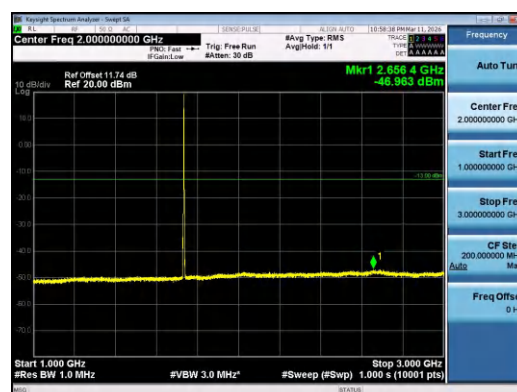
Band4-3MHz-16QAM-20175-1RB#14-1000~3000-PAS
