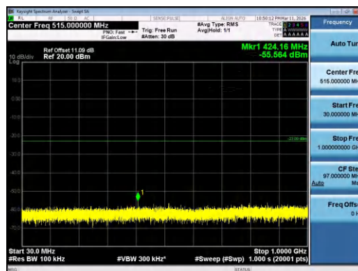
Band4-3MHz-16QAM-19965-1RB#0-30~1000-PASS
