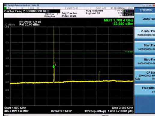
Band4-5MHz-QPSK-19975-1RB#0-1000~3000-PASS
