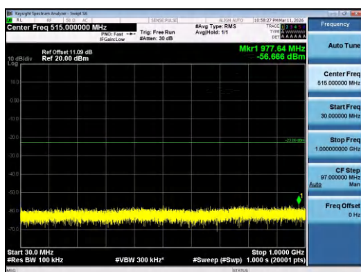
Band4-3MHz-16QAM-20175-1RB#14-30~1000-PASS
