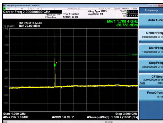
Band4-3MHz-16QAM-19965-1RB#0-1000~3000-PAS
