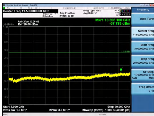
Band4-5MHz-QPSK-19975-1RB#0-3000~20000-PASS
