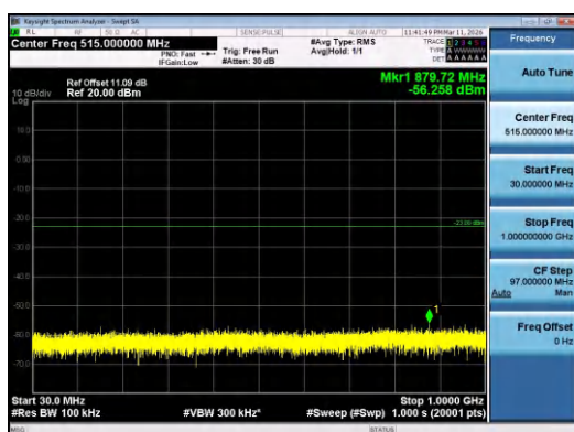
Band4-5MHz-16QAM-20175-1RB#24-30~1000-PASS
