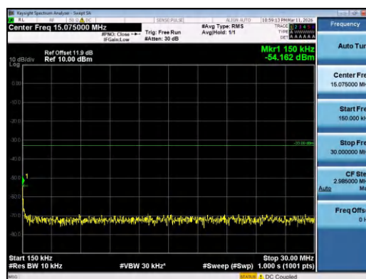
Band4-3MHz-QPSK-20175-15RB#0-0.15~30-PASS
