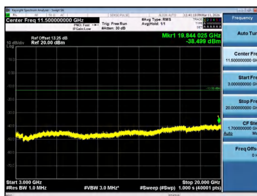
Band4-5MHz-QPSK-20175-1RB#24-3000~20000-PASS
