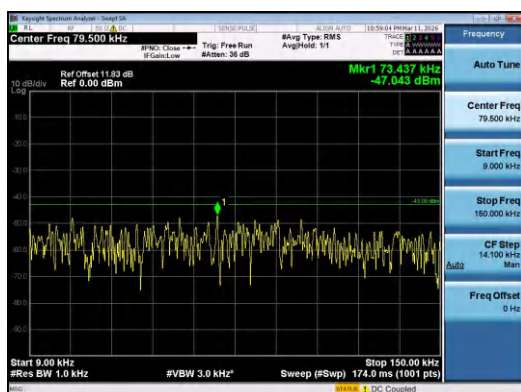
Band4-3MHz-QPSK-20175-15RB#0-0.009~0.15-PASS
