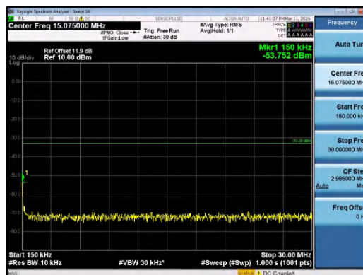
Band4-5MHz-16QAM-20175-1RB#24-0.15~30-PASS
