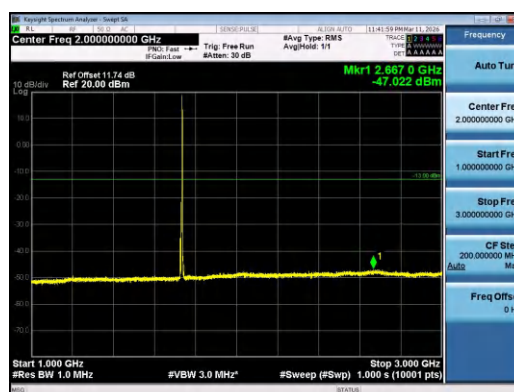
Band4-5MHz-16QAM-20175-1RB#24-1000~3000-PAS
