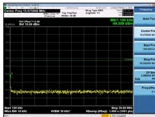
Band4-3MHz-16QAM-20175-1RB#14-0.15~30-PASS
