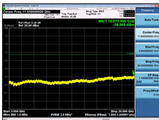
Band4-3MHz-16QAM-20175-1RB#14-3000~20000-PA
