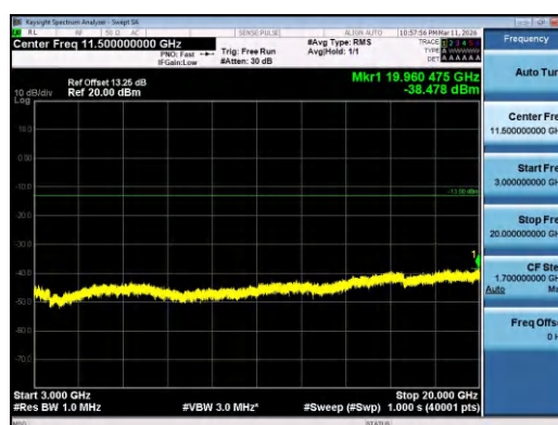
Band4-3MHz-QPSK-20175-1RB#14-3000~20000-PASS
