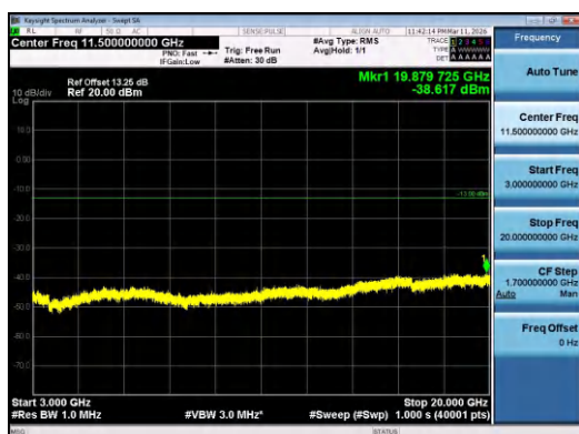
Band4-5MHz-16QAM-20175-1RB#24-3000~20000-PA
