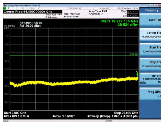
Band4-3MHz-16QAM-19965-1RB#0-3000~20000-PAS
