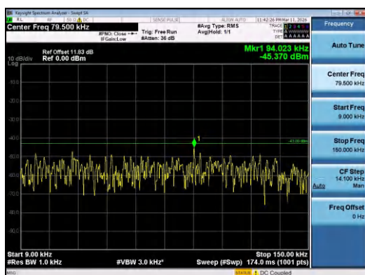
Band4-5MHz-QPSK-20175-25RB#0-0.009~0.15-PASS
