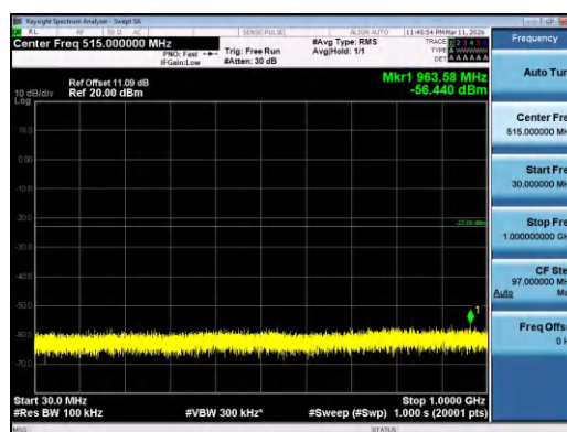
Band4-5MHz-QPSK-20175-1RB#24-30~1000-PASS
