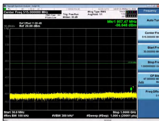
Band4-3MHz-QPSK-20175-1RB#14-30~1000-PASS
