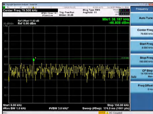
Band4-5MHz-QPSK-19975-1RB#0-0.009~0.15-PASS
