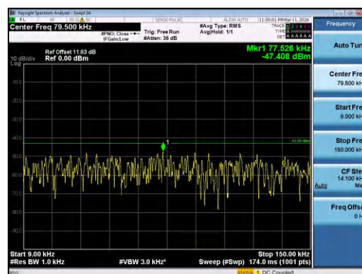
Band4-3MHz-16QAM-20175-15RB#0-0.009~0.15-PAS
