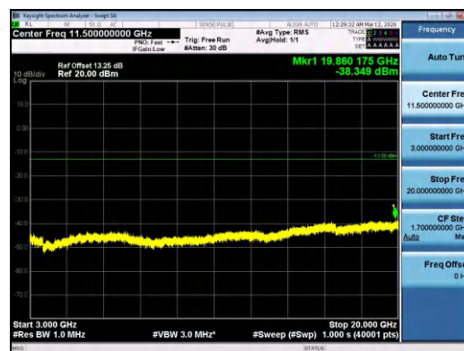
Band4-10MHz-QPSK-20350-1RB#49-3000~20000-PA
