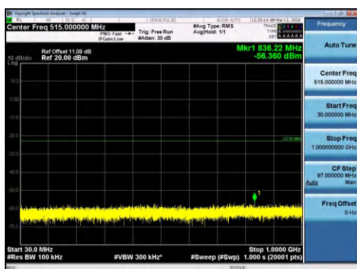
Band4-10MHz-QPSK-20175-50RB#0-30~1000-PASS
