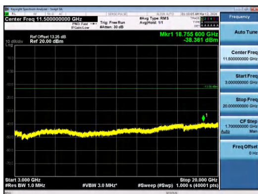
Band4-15MHz-QPSK-20175-75RB#0-3000~20000-PA
