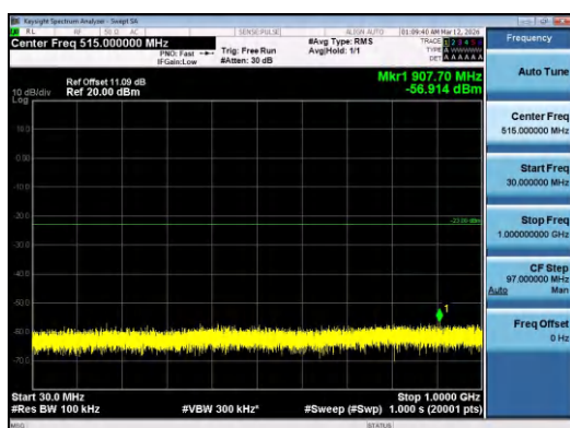
Band4-15MHz-QPSK-20175-75RB#0-30~1000-PASS
