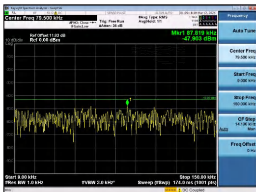
Band4-15MHz-QPSK-20175-75RB#0-0.009~0.15-PAS
