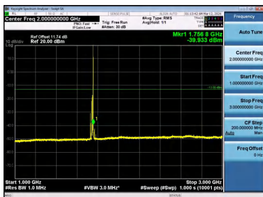
Band4-15MHz-QPSK-20325-1RB#74-1000~3000-PAS
