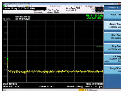
Band4-15MHz-QPSK-20175-75RB#0-0.15~30-PASS
