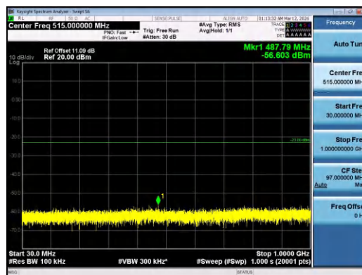
Band4-15MHz-QPSK-20325-1RB#74-30~1000-PASS
