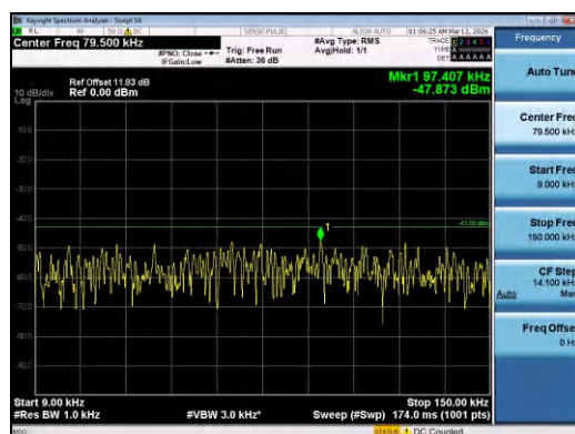
Band4-15MHz-16QAM-20175-1RB#0-0.009~0.15-PAS
