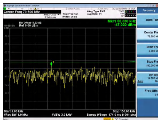
Band4-10MHz-16QAM-20175-1RB#0-0.009~0.15-PAS
