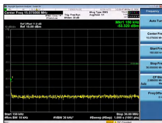
Band4-10MHz-QPSK-20350-50RB#0-0.15~30-PASS
