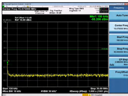
Band4-15MHz-QPSK-20325-1RB#74-0.15~30-PASS
