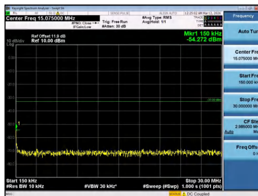
Band4-10MHz-QPSK-20175-50RB#0-0.15~30-PASS
