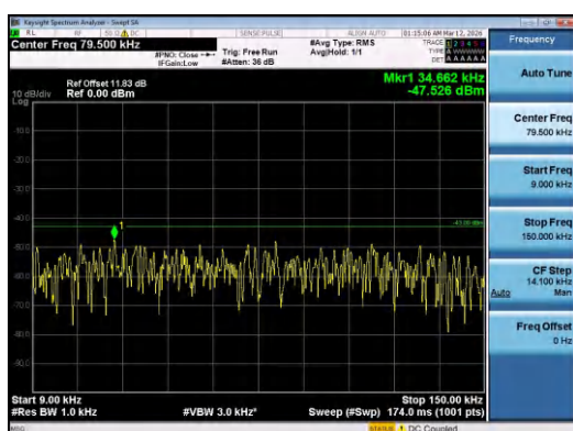
Band4-15MHz-QPSK-20325-75RB#0-0.009~0.15-PAS
