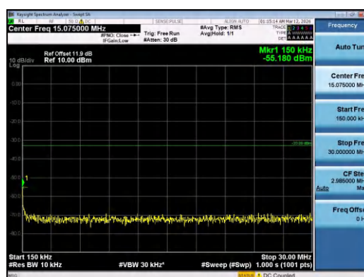
Band4-15MHz-QPSK-20325-75RB#0-0.15~30-PASS
