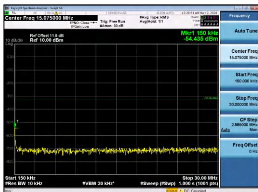
Band4-10MHz-QPSK-20350-1RB#49-0.15~30-PASS
