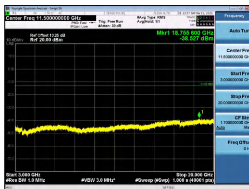
Band4-15MHz-QPSK-20325-1RB#74-3000~20000-PASS
