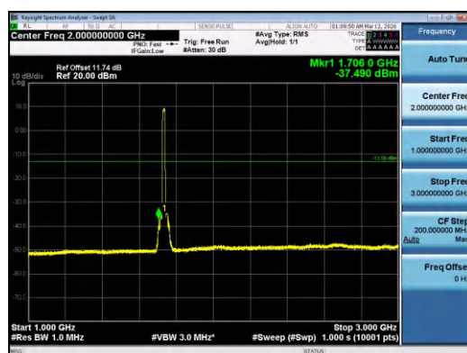
Band4-15MHz-QPSK-20175-75RB#0-1000~3000-PAS
