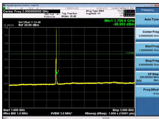
Band4-10MHz-QPSK-20350-1RB#49-1000~3000-PAS
