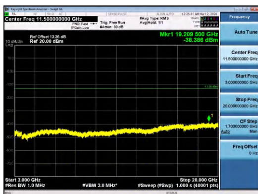
Band4-10MHz-QPSK-20175-50RB#0-3000~20000-PA
