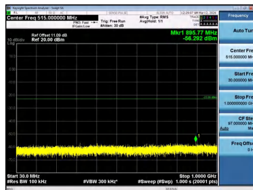
Band4-10MHz-QPSK-20350-1RB#49-30~1000-PASS
