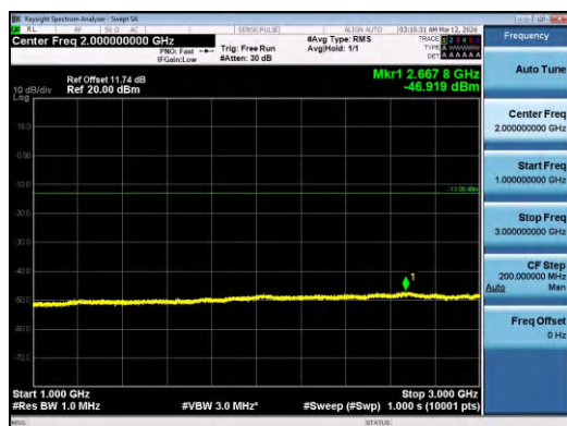
Band5-3MHz-16QAM-20415-1RB#0-1000~3000-PAS
