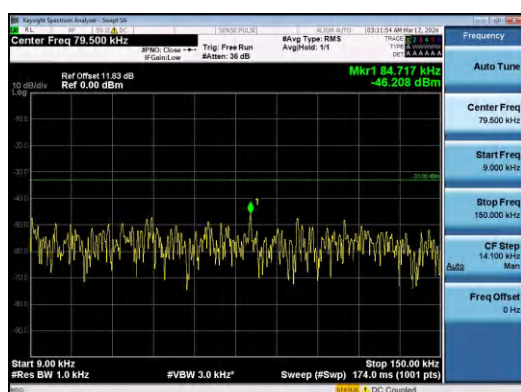
Band5-3MHz-16QAM-20415-1RB#14-0.009~0.15-PAS
