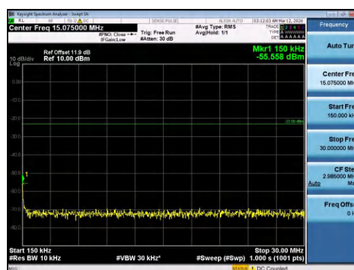
Band5-3MHz-16QAM-20415-1RB#14-0.15~30-PASS
