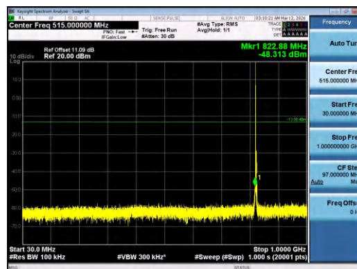
Band5-3MHz-16QAM-20415-1RB#0-30~1000-PASS
