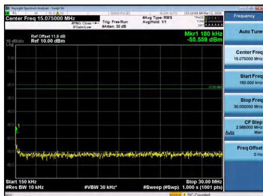
Band5-3MHz-16QAM-20415-1RB#0-0.15~30-PASS
