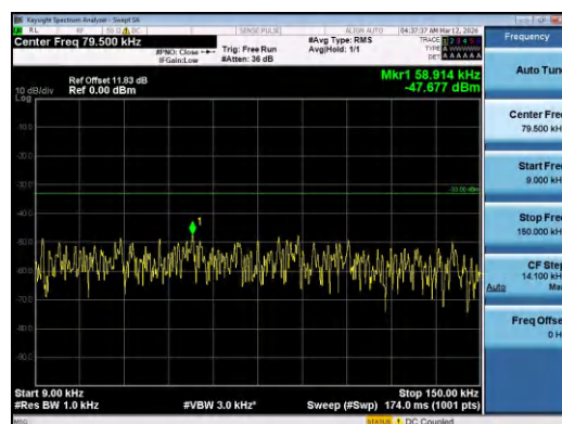
Band5-10MHz-16QAM-20525-1RB#0-0.009~0.15-PAS
