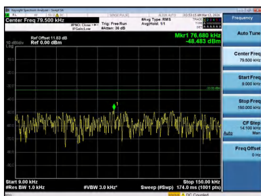
Band5-5MHz-16QAM-20425-1RB#24-0.009~0.15-PAS
