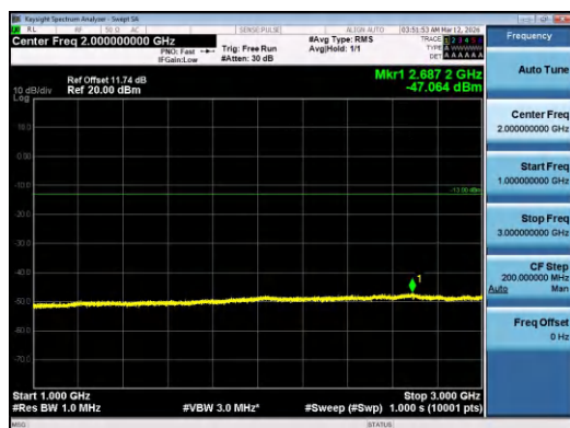
Band5-5MHz-16QAM-20425-1RB#0-1000~3000-PAS
