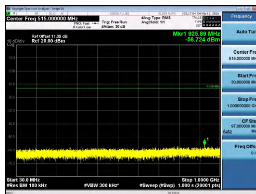
Band5-3MHz-QPSK-20525-1RB#14-30~1000-PASS
