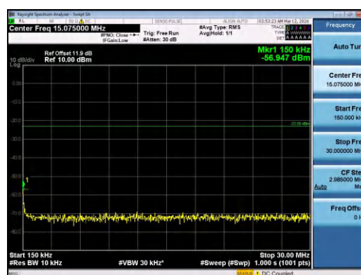
Band5-5MHz-16QAM-20425-1RB#24-0.15~30-PASS
