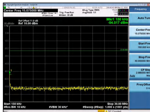
Band5-10MHz-QPSK-20525-50RB#0-0.15~30-PASS
