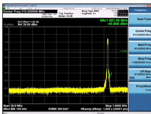
Band5-10MHz-QPSK-20525-50RB#0-30~1000-PASS
