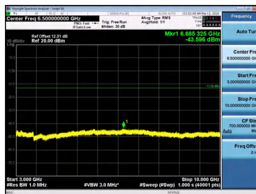
Band5-5MHz-16QAM-20425-1RB#0-3000~10000-PAS
