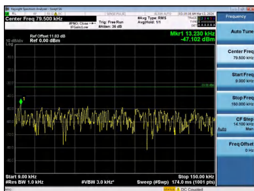
Band5-3MHz-QPSK-20525-15RB#0-0.009~0.15-PASS
