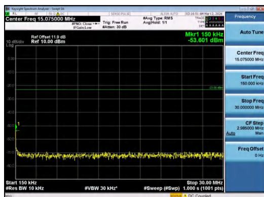
Band5-3MHz-QPSK-20525-1RB#14-0.15~30-PASS
