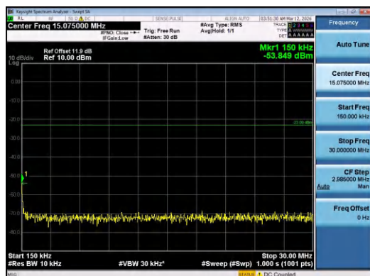
Band5-5MHz-16QAM-20425-1RB#0-0.15~30-PASS
