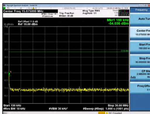
Band5-5MHz-QPSK-20525-25RB#0-0.15~30-PASS
