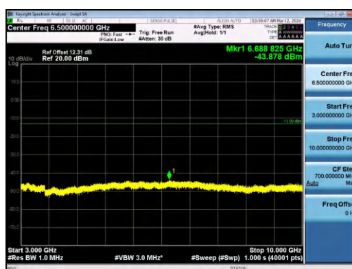
Band5-5MHz-QPSK-20525-1RB#24-3000~10000-PASS
