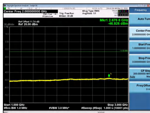
Band5-10MHz-QPSK-20525-50RB#0-1000~3000-PAS
