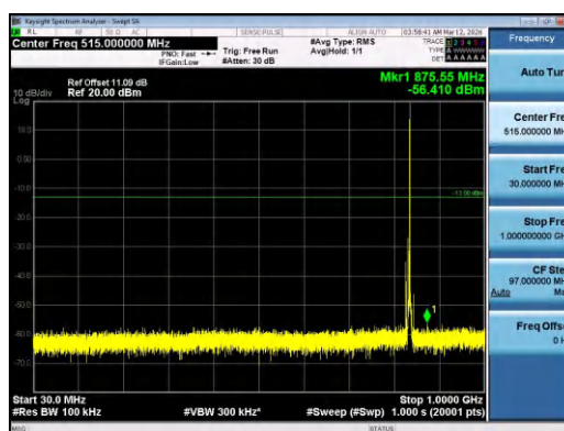
Band5-5MHz-QPSK-20525-1RB#24-30~1000-PASS
