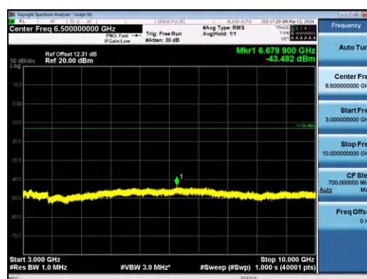
Band5-3MHz-QPSK-20525-1RB#14-3000~10000-PASS
