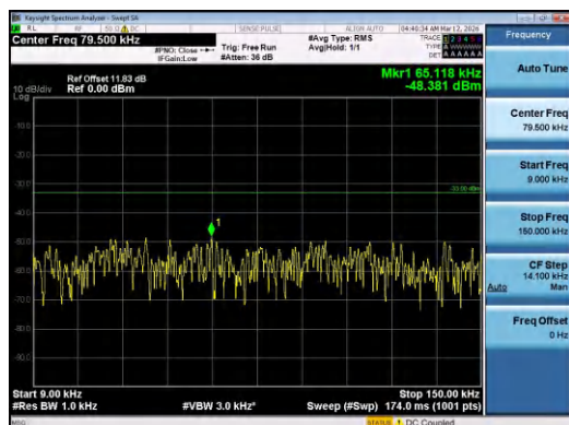
Band5-10MHz-QPSK-20525-50RB#0-0.009~0.15-PAS
