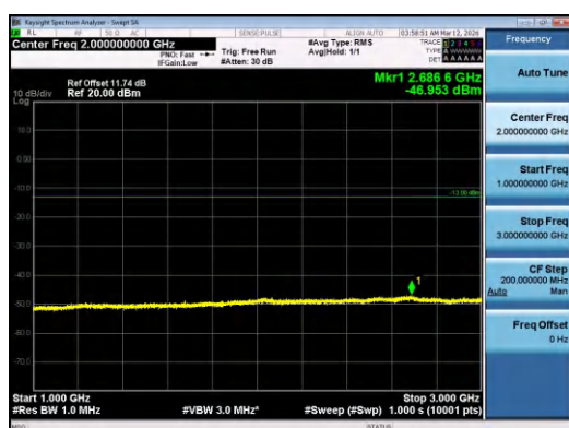
Band5-5MHz-QPSK-20525-1RB#24-1000~3000-PASS
