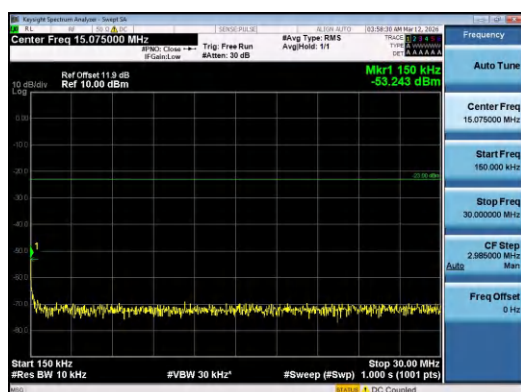
Band5-5MHz-QPSK-20525-1RB#24-0.15~30-PASS
