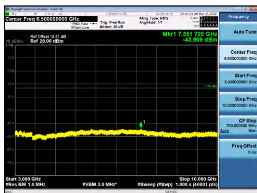
Band5-10MHz-QPSK-20525-50RB#0-3000~10000-PA
