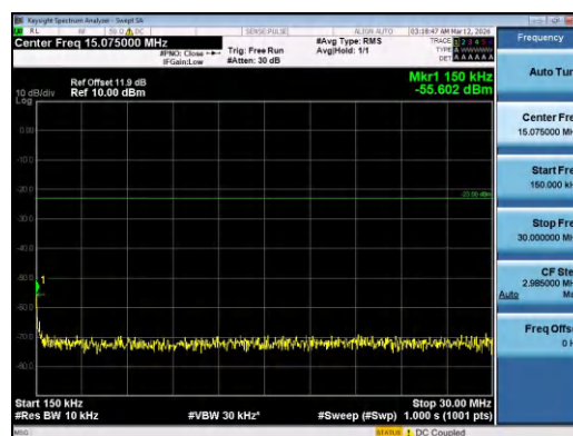
Band5-3MHz-QPSK-20525-15RB#0-0.15~30-PASS
