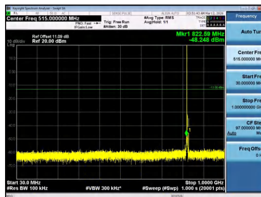
Band5-5MHz-16QAM-20425-1RB#0-30~1000-PASS
