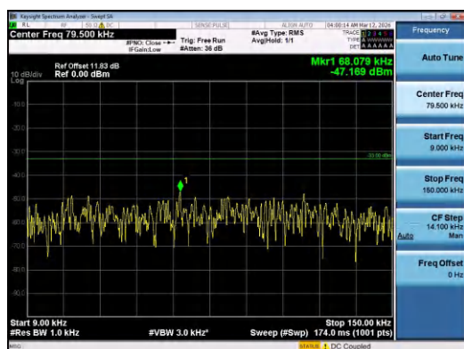
Band5-5MHz-QPSK-20525-25RB#0-0.009~0.15-PASS
