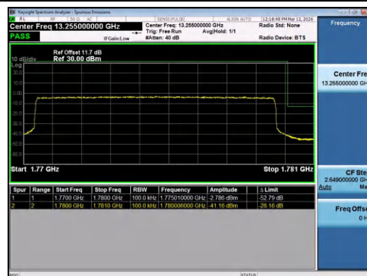
Band66-10MHz-16QAM-132622-50RB#0-PASS
