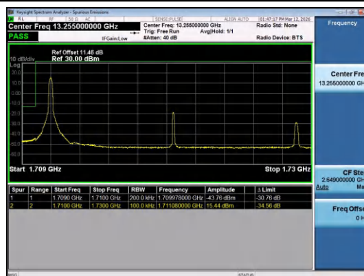
Band66-20MHz-16QAM-132072-1RB#0-PASS
