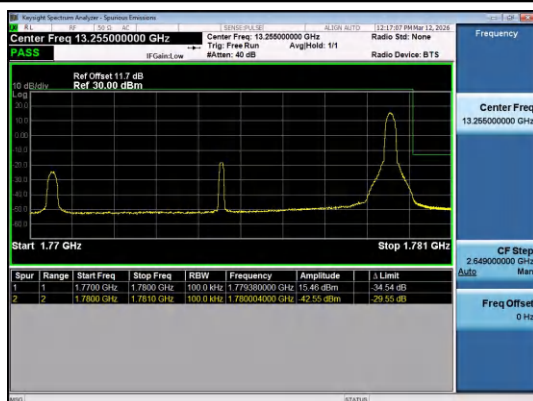
Band66-10MHz-16QAM-132622-1RB#49-PASS
