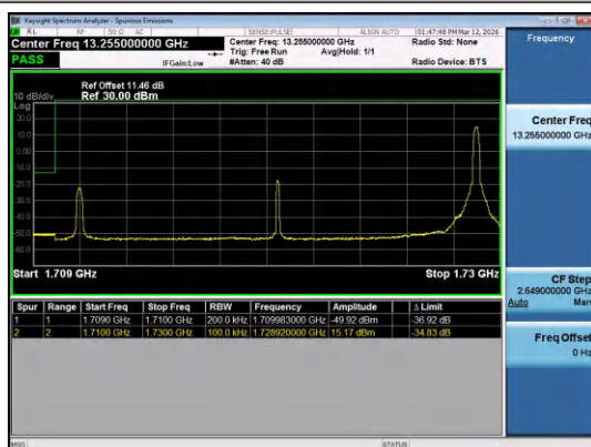
Band66-20MHz-16QAM-132072-1RB#99-PASS
