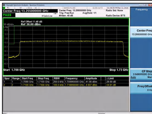
Band66-20MHz-QPSK-132072-100RB#0-PASS
