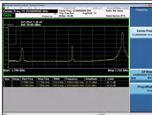
Band66-15MHz-16QAM-132047-1RB#74-PASS
