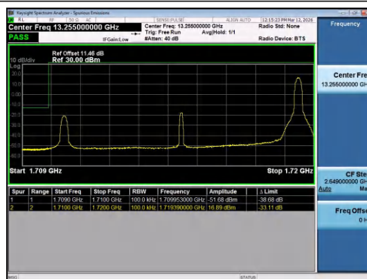
Band66-10MHz-QPSK-132022-1RB#49-PASS
