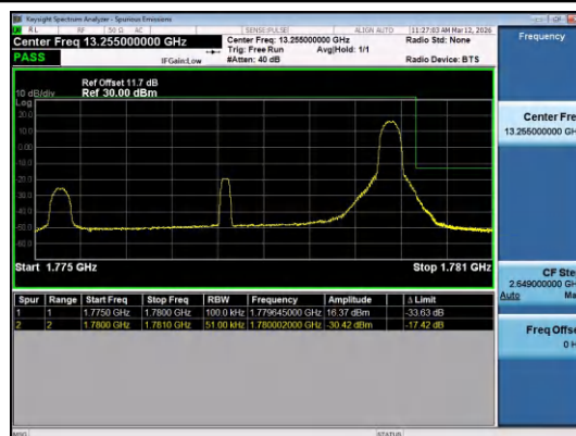
Band66-5MHz-QPSK-132647-1RB#24-PASS
