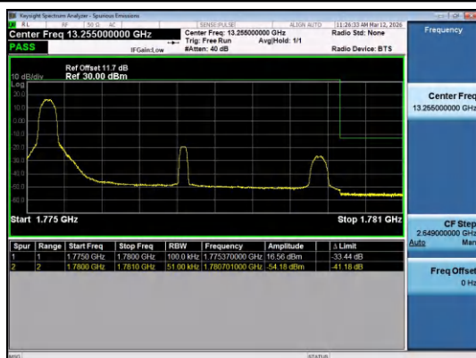
Band66-5MHz-QPSK-132647-1RB#0-PASS
