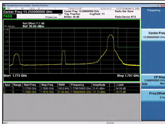
Band66-5MHz-16QAM-132647-1RB#24-PASS
