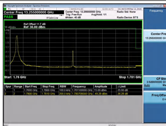
Band66-20MHz-16QAM-132572-1RB#0-PASS
