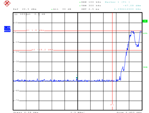
Hopping mode
