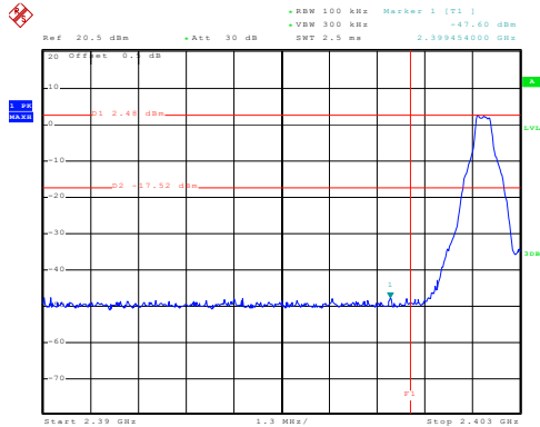
No-hopping mode
