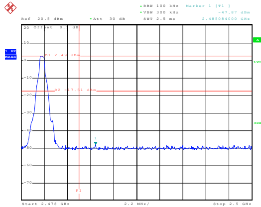
No-hopping mode
