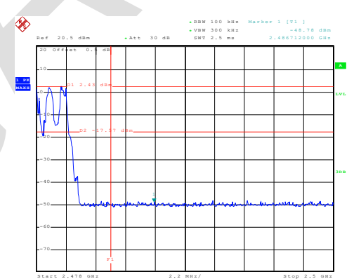
Hopping mode
