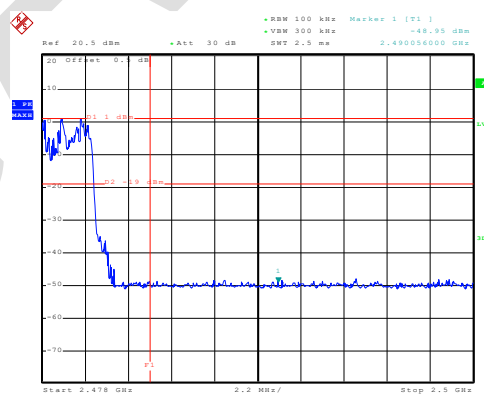
Hopping mode
