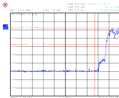
Hopping mode
