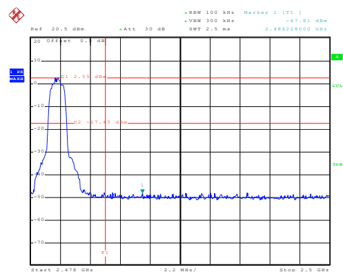
No-hopping mode
