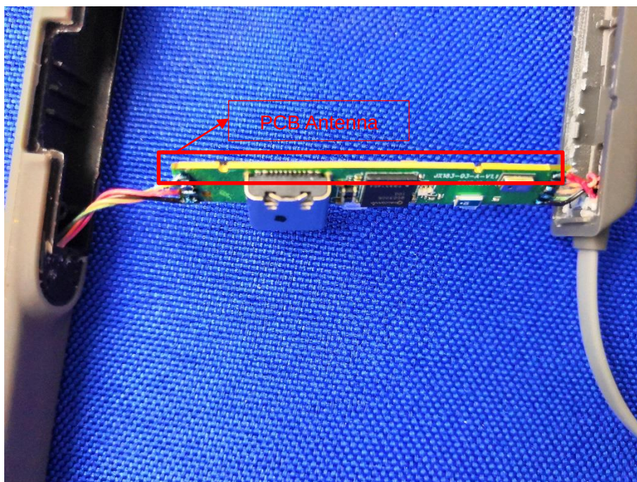
ANTENNA CLOSE-UP 1
