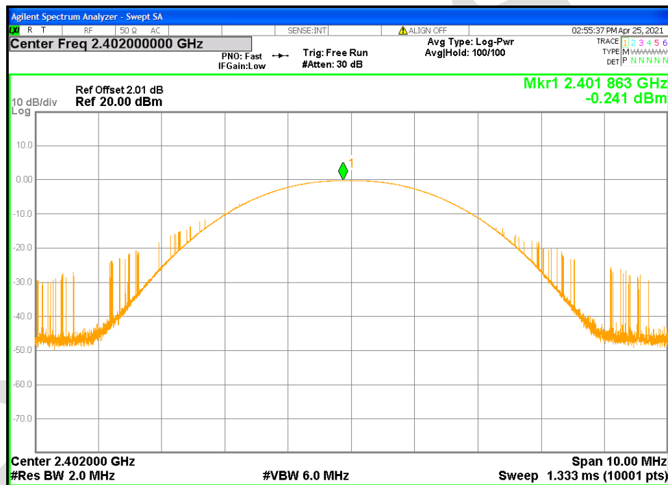
Power NVNT 1-DH1 2402MHz Ant1
