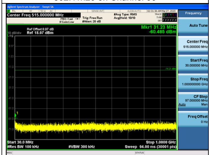
802.11n20 on Channel 06
