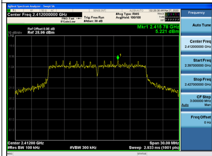
802.11n20 on Channel 01
