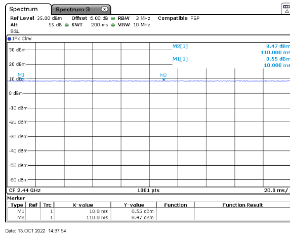
Figure 6: Pulsed Emission Characteristics (Duty Cycle).
