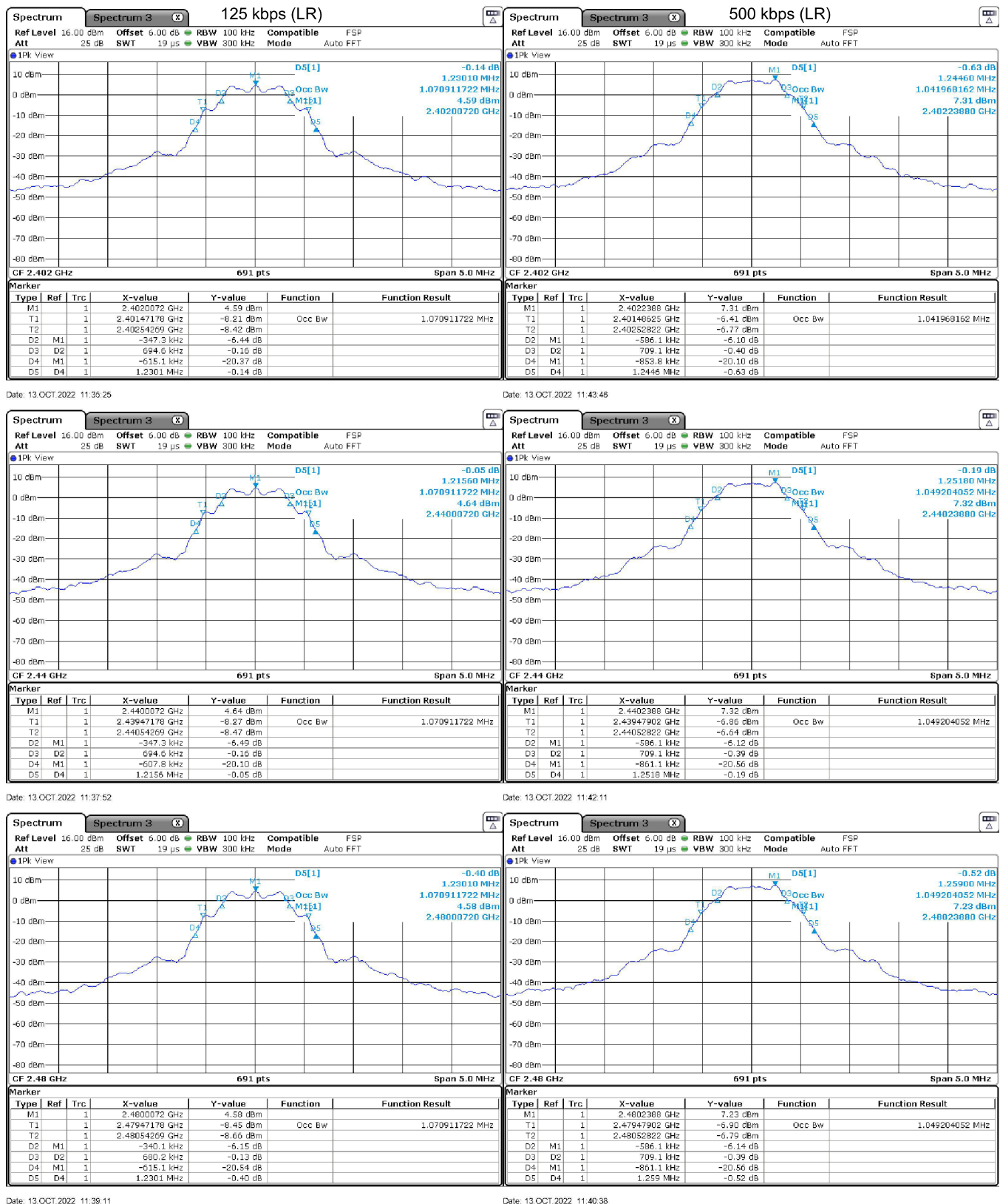
Figure 7(a): Example Intentional Emission Bandwidth Plots.
