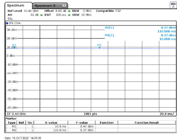
Figure 6: Pulsed Emission Characteristics (Duty Cycle).
