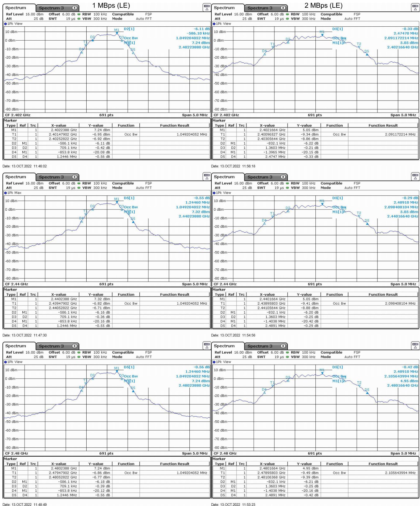
Figure 7(b): Example Intentional Emission Bandwidth Plots.
