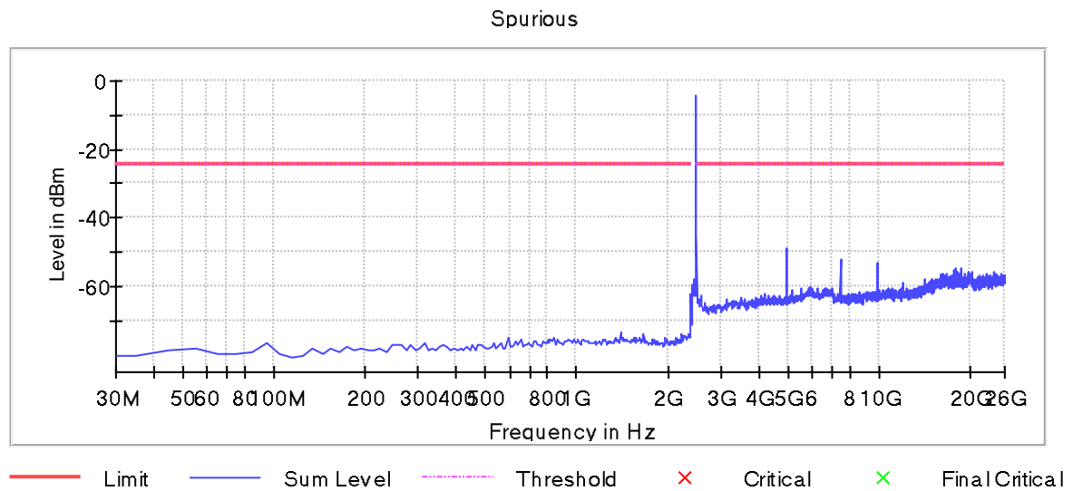
Plot 22: Mode 1, CSE, high channel
