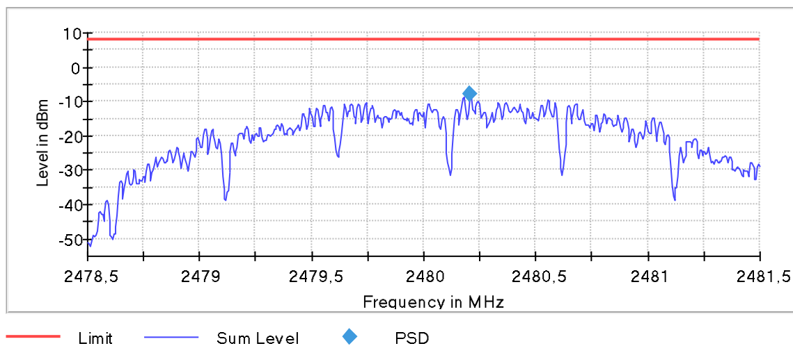
Plot 15: Mode 1, Peak PSD, high channel
