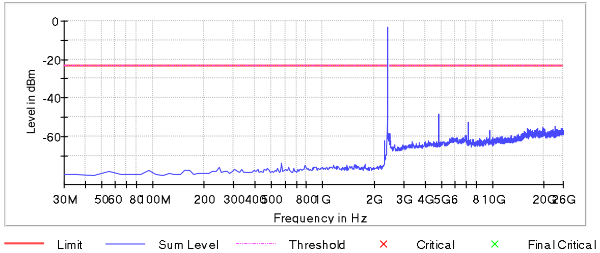
Plot 20: Mode 1, CSE, low channel
