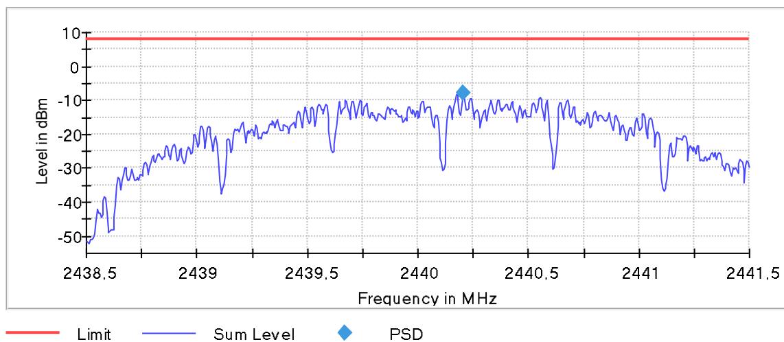
Plot 14: Mode 1, Peak PSD, mid channel
