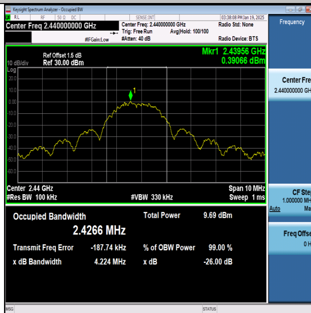
Thread-Ant1-2440
