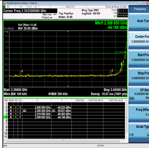
Thread-Ant1-2405-PASS
