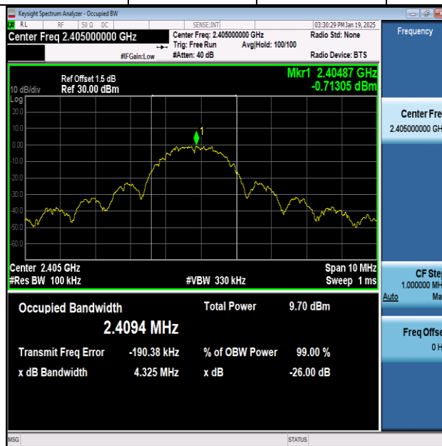
Thread-Ant1-2405
