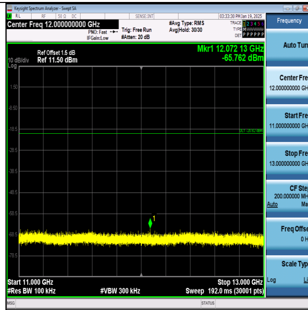
Thread-Ant1-2405-11000~13000-PASS
