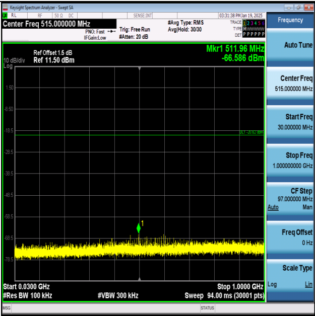
Thread-Ant1-2405-30~1000-PASS
