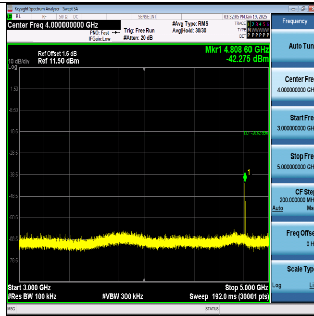
Thread-Ant1-2405-3000-5000-PASS
