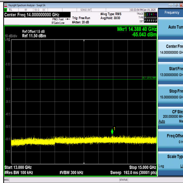
Thread-Ant1-2405-13000~15000-PASS
