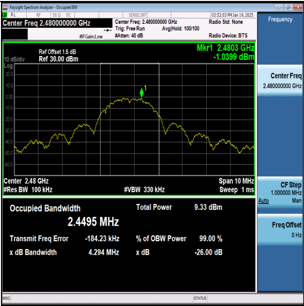
Thread-Ant1-2480
