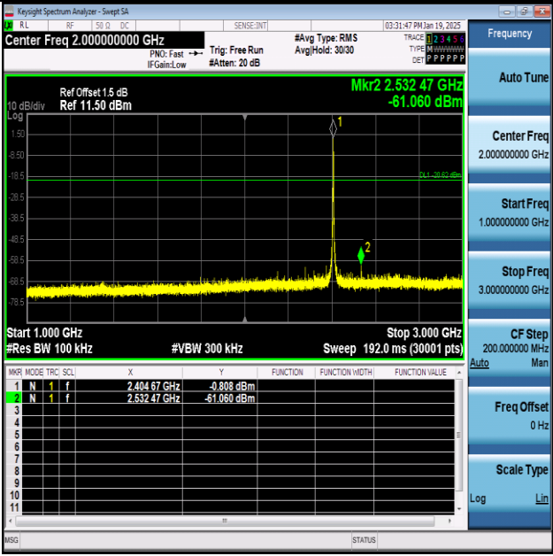
Thread-Ant1-2405-1000~3000-PASS
