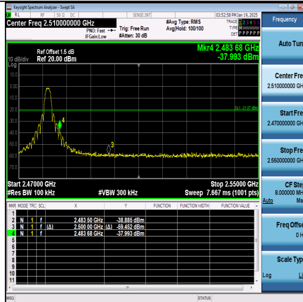
Thread-Ant1-2480-PASS
