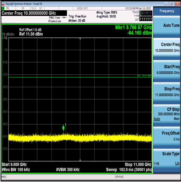
Thread-Ant1-2405-9000-11000-PASS
