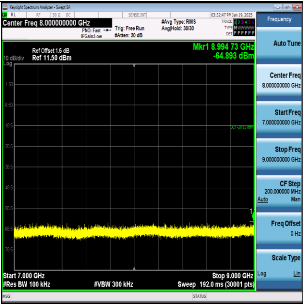
Thread-Ant1-2405-7000-9000-PASS
