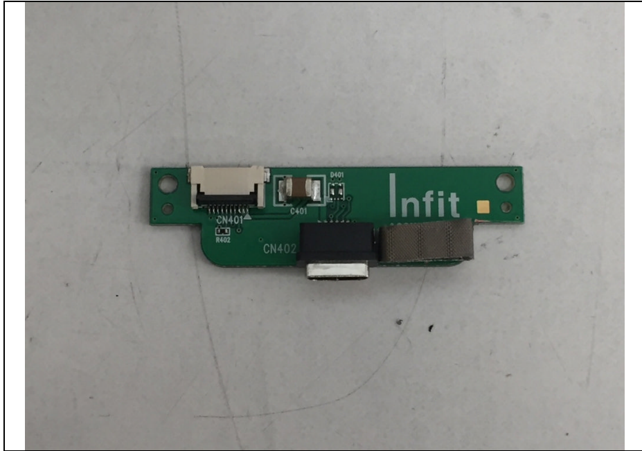
Top view of Sub PCB 1
