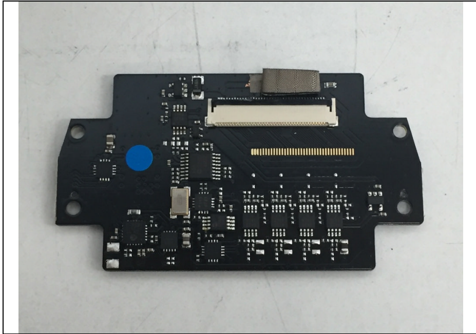
Top view of Sub PCB 2
