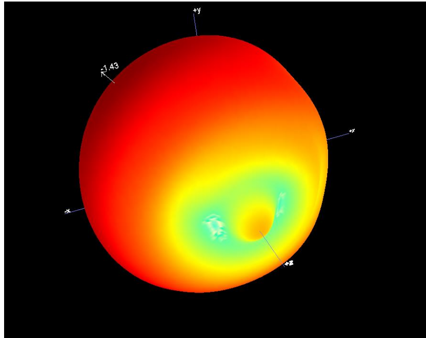
B1.1 3D Pattern for 2400MHz
