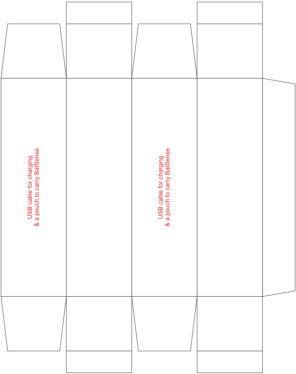
CHARGER BOX
