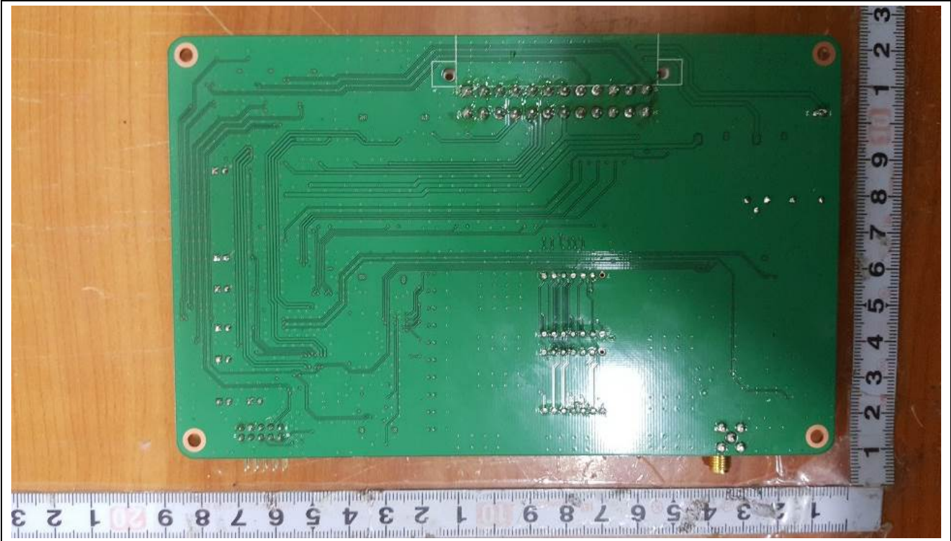
MainBoard-Rear
