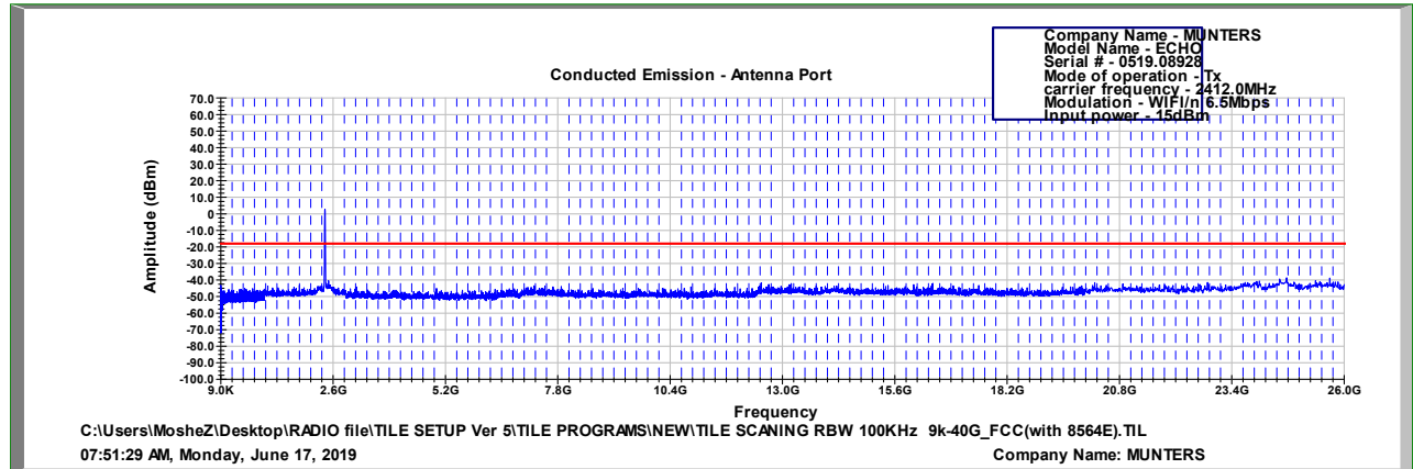
Figure 122 2412.0 MHz, WI-FI/n(6.5Mbit/s)
