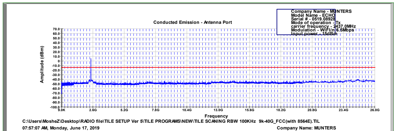
Figure 123 2437.0 MHz, WI-FI/n(6.5Mbit/s)
