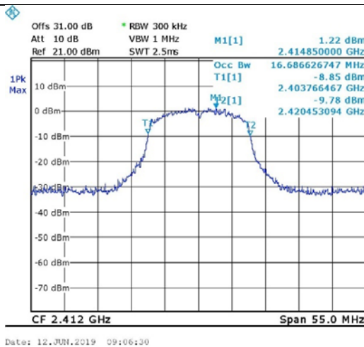
Figure 97. 2412.0 MHz, Wi-fi/g(6Mbit/s)
