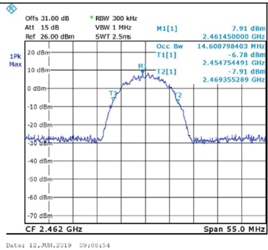
Figure 96. 2462.0 MHz, Wi-fi/b(11Mbit/s)
