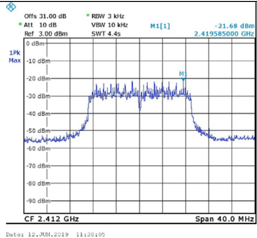
Figure 84. 2412.0 MHz, Wi-fi/n(65Mbit/s)
