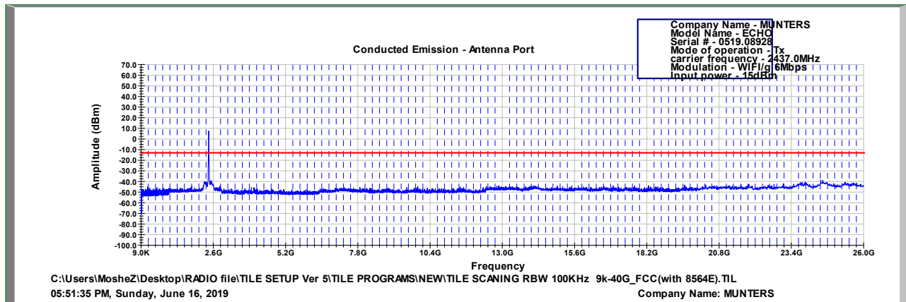
Figure 117 2437.0 MHz, WI-FI/g(6Mbit/s)
