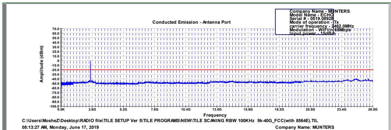
Figure 127 2462.0 MHz, WI-FI/n(65Mbit/s)
