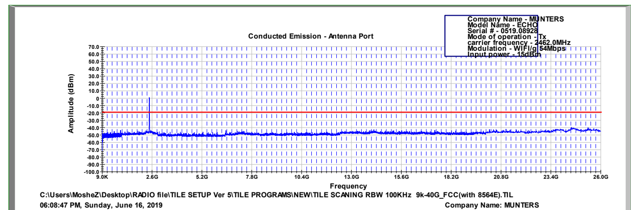
Figure 121 2462.0 MHz, WI-FI/g(54Mbit/s)
