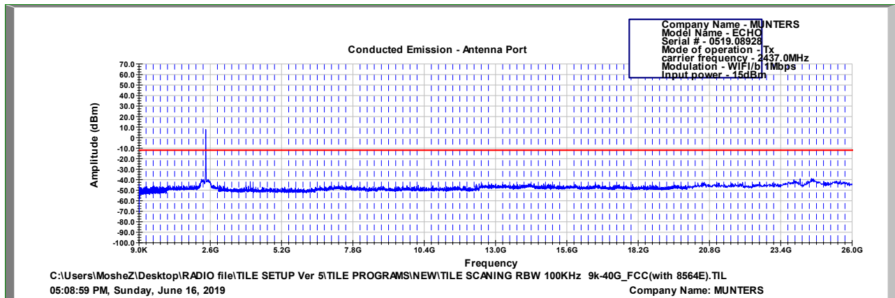
Figure 111 2437.0 MHz, WI-FI/b(1Mbit/s)
