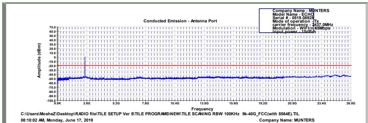
Figure 126 2437.0 MHz, WI-FI/n(65Mbit/s)
