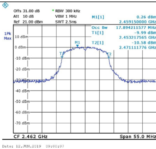
Figure 107. 2462.0 MHz, Wi-fi/n(6.5Mbit/s)
