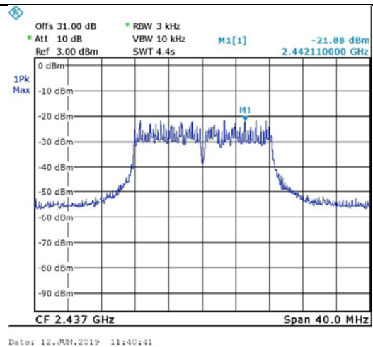
Figure 80. 2437.0 MHz, Wi-fi/g(54Mbit/s)
