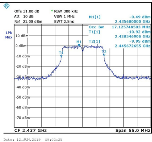
Figure 100. 2437.0 MHz, Wi-fi/g(54Mbit/s)
