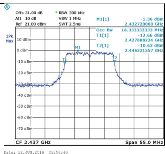
Figure 106. 2437.0 MHz, Wi-fi/n(65Mbit/s)
