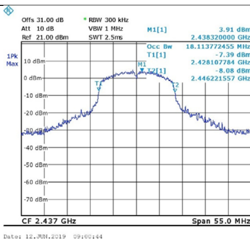
Figure 105. 2437.0 MHz, Wi-fi/n(6.5Mbit/s)
