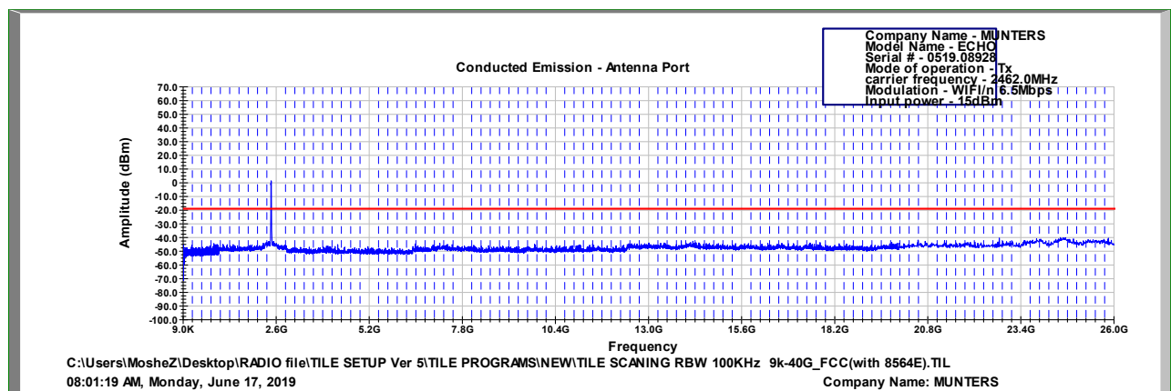
Figure 124 2462.0 MHz, WI-FI/n(6.5Mbit/s)
