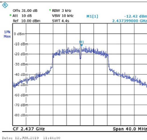
Figure 79. 2437.0 MHz, Wi-fi/g(6Mbit/s)
