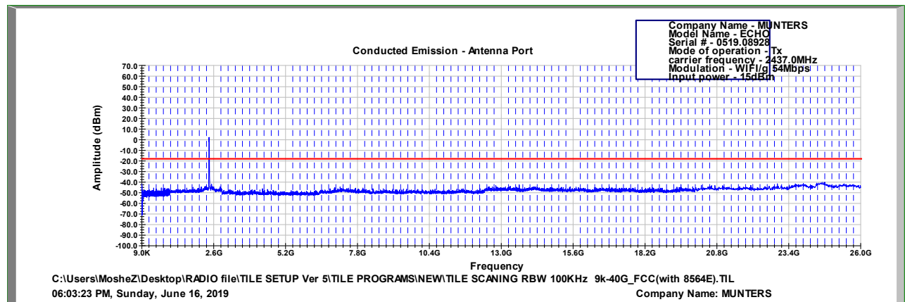
Figure 120 2437.0 MHz, WI-FI/g(54Mbit/s)
