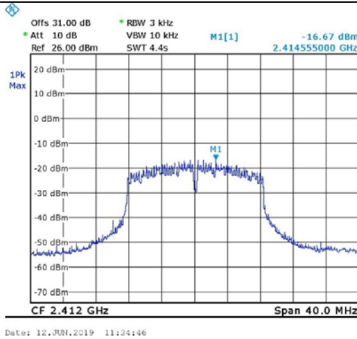
Figure 77. 2412.0 MHz, Wi-fi/g(6Mbit/s)
