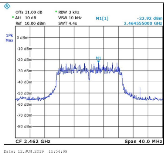
Figure 88. 2462.0 MHz, Wi-fi/n(65Mbit/s)
