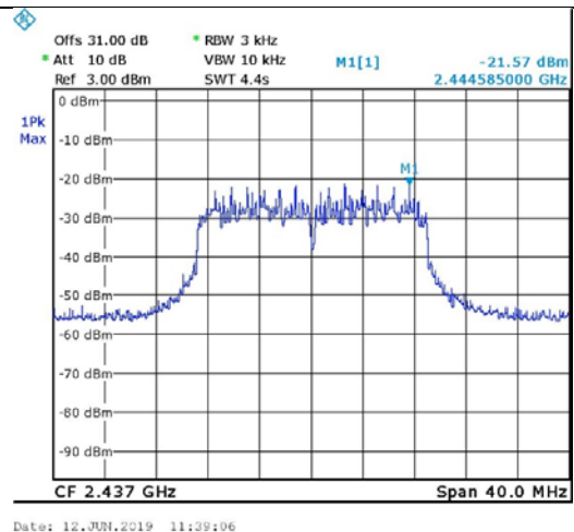
Figure 86. 2437.0 MHz, Wi-fi/n(65Mbit/s)
