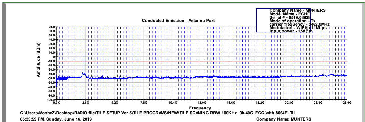
Figure 115 2462.0 MHz, WI-FI/b(11Mbit/s)
