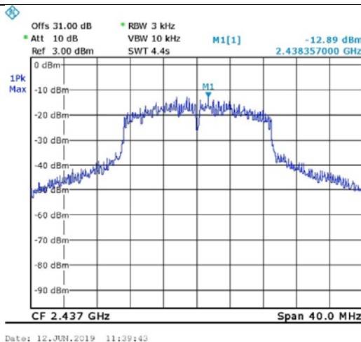
Figure 85. 2437.0 MHz, Wi-fi/n(6.5Mbit/s)
