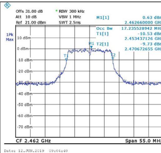
Figure 102. 2462.0 MHz, Wi-fi/g(54Mbit/s)
