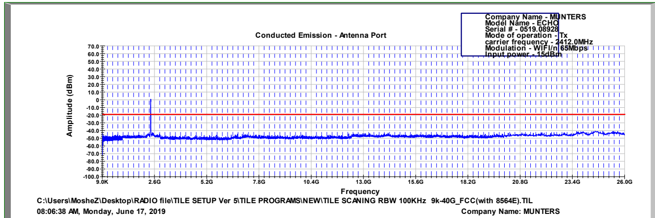
Figure 125 2412.0 MHz, WI-FI/n(65Mbit/s)
