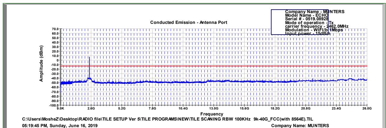
Figure 112 2462.0 MHz, WI-FI/b(1Mbit/s)
