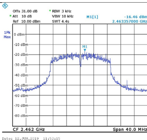
Figure 87. 2462.0 MHz, Wi-fi/n(6.5Mbit/s)
