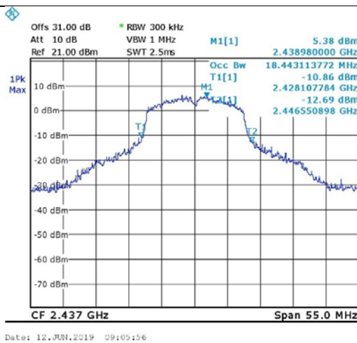
Figure 99. 2437.0 MHz, Wi-fi/g(6Mbit/s)
