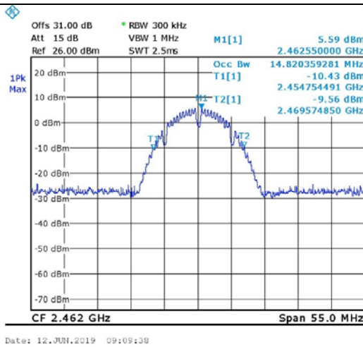
Figure 95. 2462.0 MHz, Wi-fi/b(1Mbit/s)
