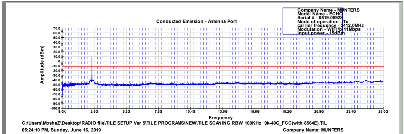
Figure 113 2412.0 MHz, WI-FI/b(11Mbit/s)
