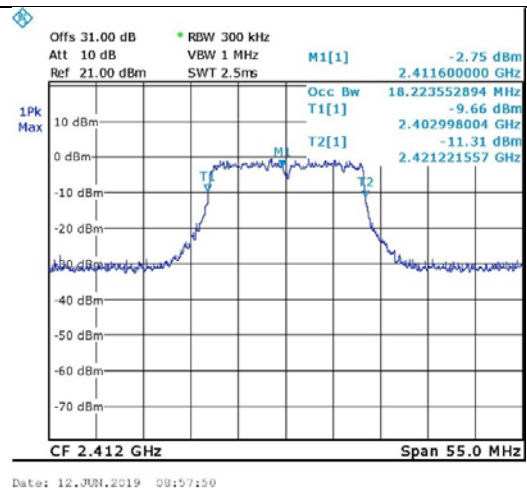
Figure 104. 2412.0 MHz, Wi-fi/n(65Mbit/s)
