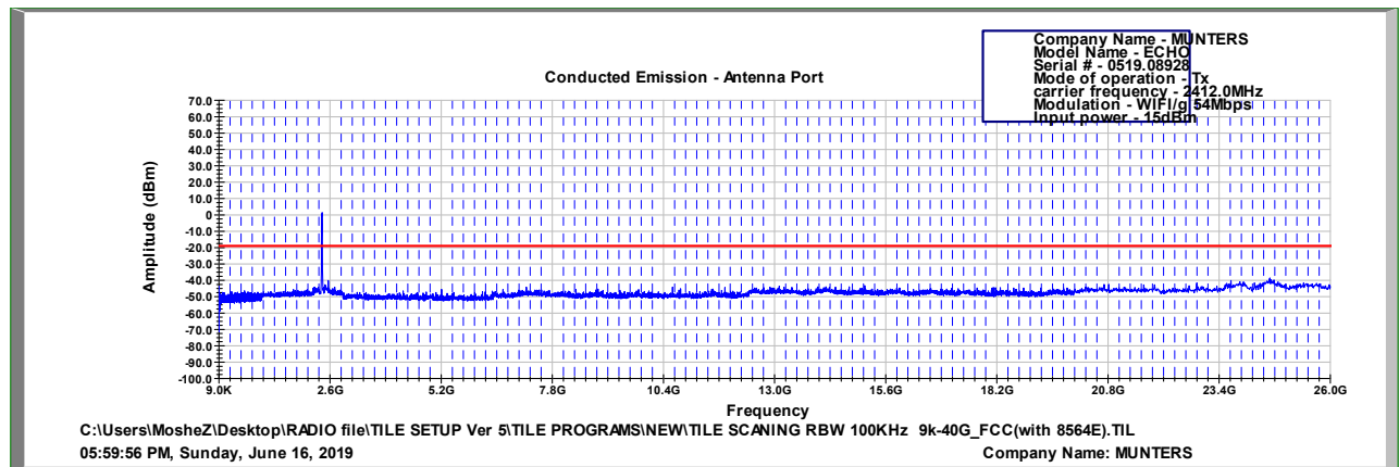
Figure 119 2412.0 MHz, WI-FI/g(54Mbit/s)
