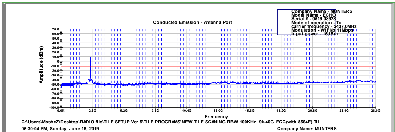
Figure 114 2437.0 MHz, WI-FI/b(11Mbit/s)
