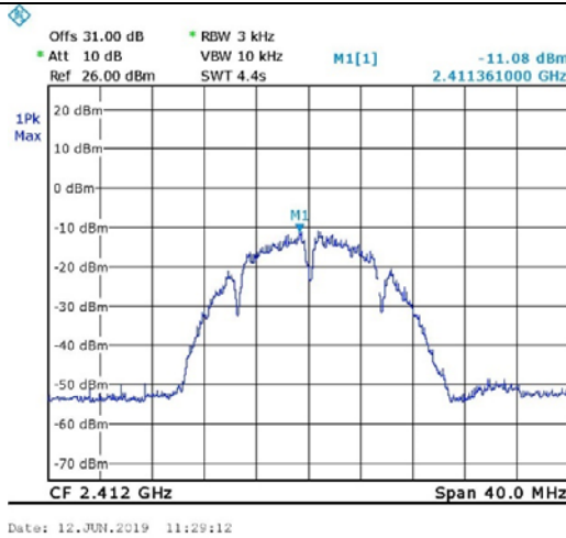
Figure 71. 2412.0 MHz, Wi-fi/b(1Mbit/s)
