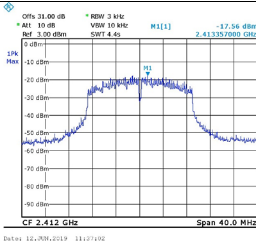
Figure 83. 2412.0 MHz, Wi-fi/n(6.5Mbit/s)
