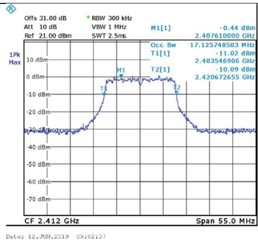
Figure 98. 2412.0 MHz, Wi-fi/g(54Mbit/s)
