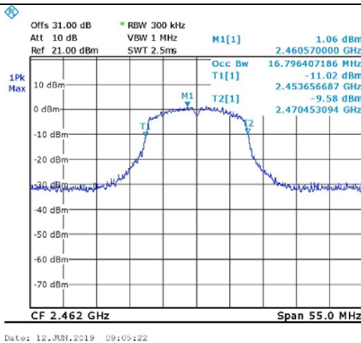
Figure 101. 2462.0 MHz, Wi-fi/g(6Mbit/s)
