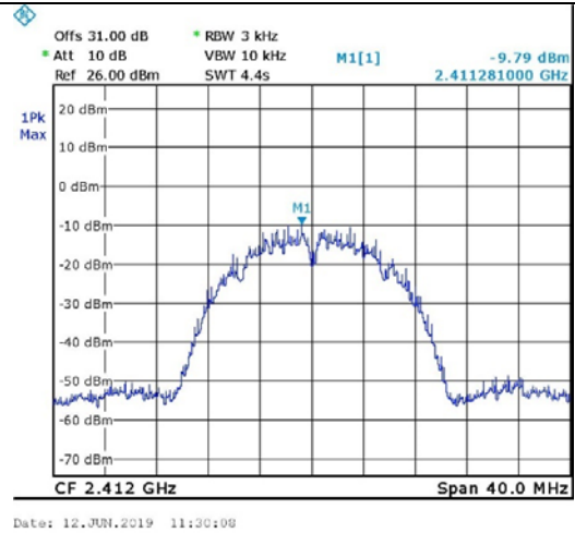
Figure 72. 2412.0 MHz, Wi-fi/b(11Mbit/s)
