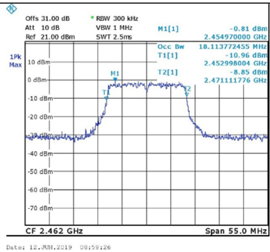
Figure 108. 2462.0 MHz, Wi-fi/n(65Mbit/s)
