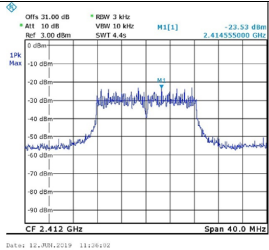
Figure 78. 2412.0 MHz, Wi-fi/g(54Mbit/s)
