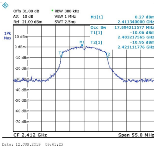
Figure 103. 2412.0 MHz, Wi-fi/n(6.5Mbit/s)
