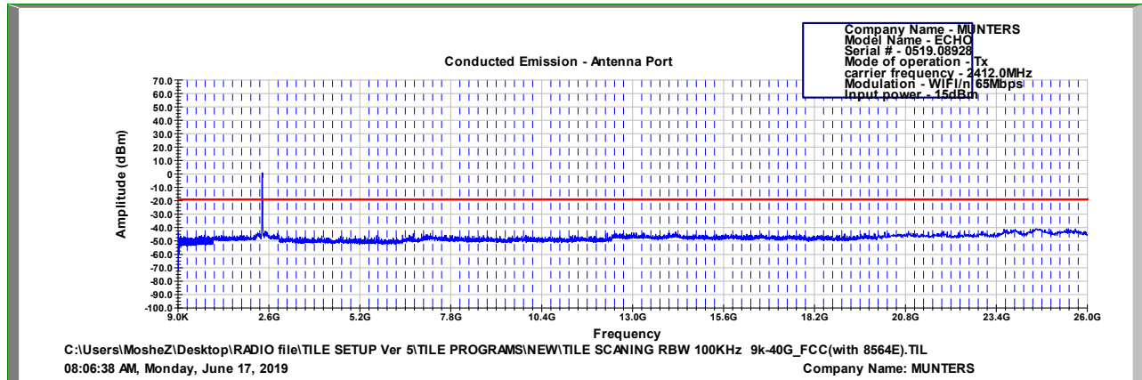
Figure 125 2412.0 MHz, WI-FI/n(65Mbit/s)
