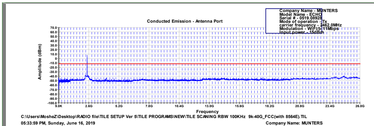
Figure 115 2462.0 MHz, WI-FI/b(11Mbit/s)
