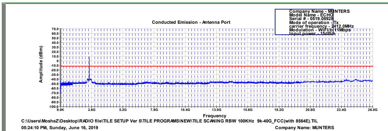
Figure 113 2412.0 MHz, WI-FI/b(11Mbit/s)
