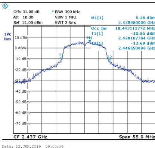
Figure 99. 2437.0 MHz, Wi-fi/g(6Mbit/s)
