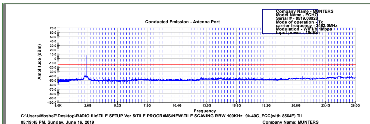
Figure 112 2462.0 MHz, WI-FI/b(1Mbit/s)
