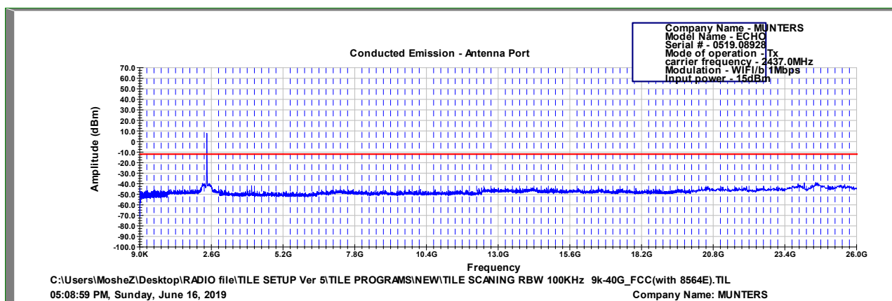
Figure 111 2437.0 MHz, WI-FI/b(1Mbit/s)
