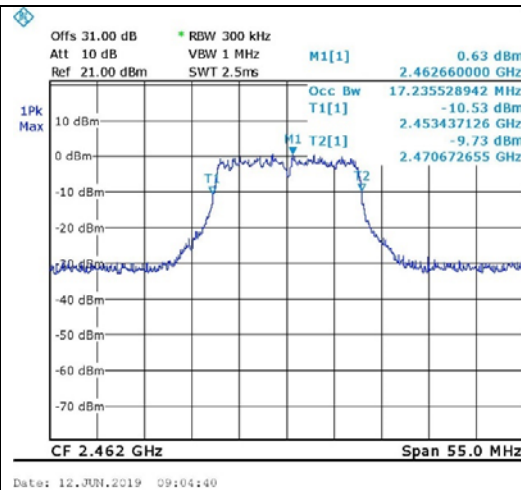
Figure 102. 2462.0 MHz, Wi-fi/g(54Mbit/s)
