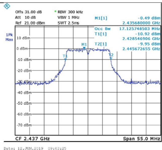
Figure 100. 2437.0 MHz, Wi-fi/g(54Mbit/s)
