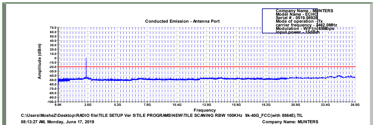
Figure 127 2462.0 MHz, WI-FI/n(65Mbit/s)
