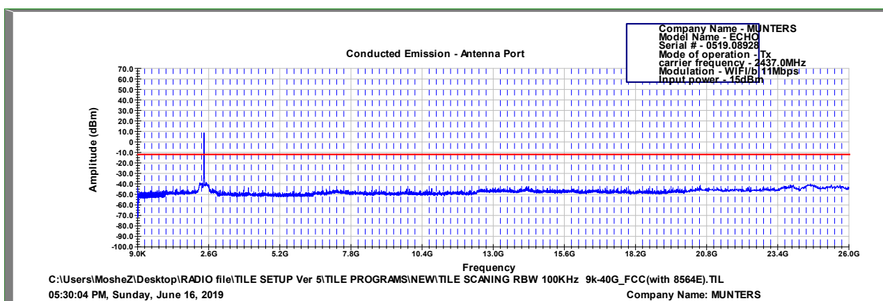
Figure 114 2437.0 MHz, WI-FI/b(11Mbit/s)
