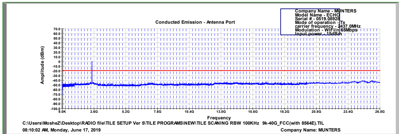
Figure 126 2437.0 MHz, WI-FI/n(65Mbit/s)
