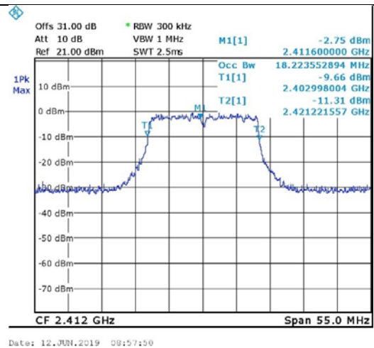
Figure 104. 2412.0 MHz, Wi-fi/n(65Mbit/s)
