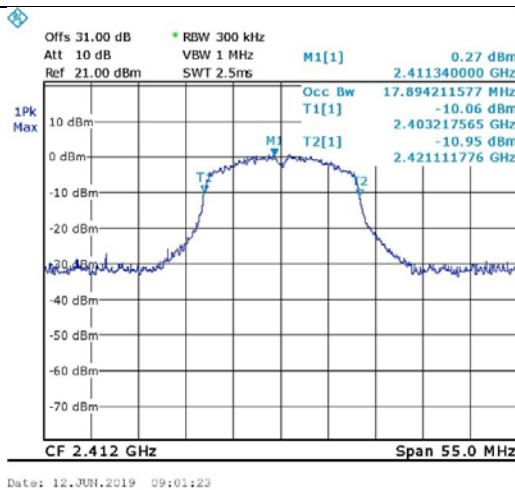
Figure 103. 2412.0 MHz, Wi-fi/n(6.5Mbit/s)
