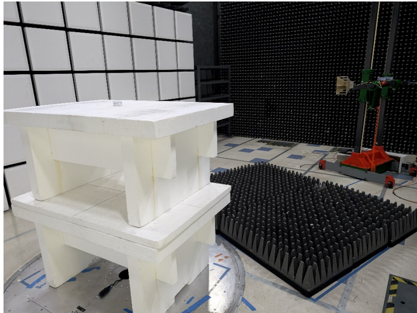
Above 1000MHz Radiated Emission Setup
