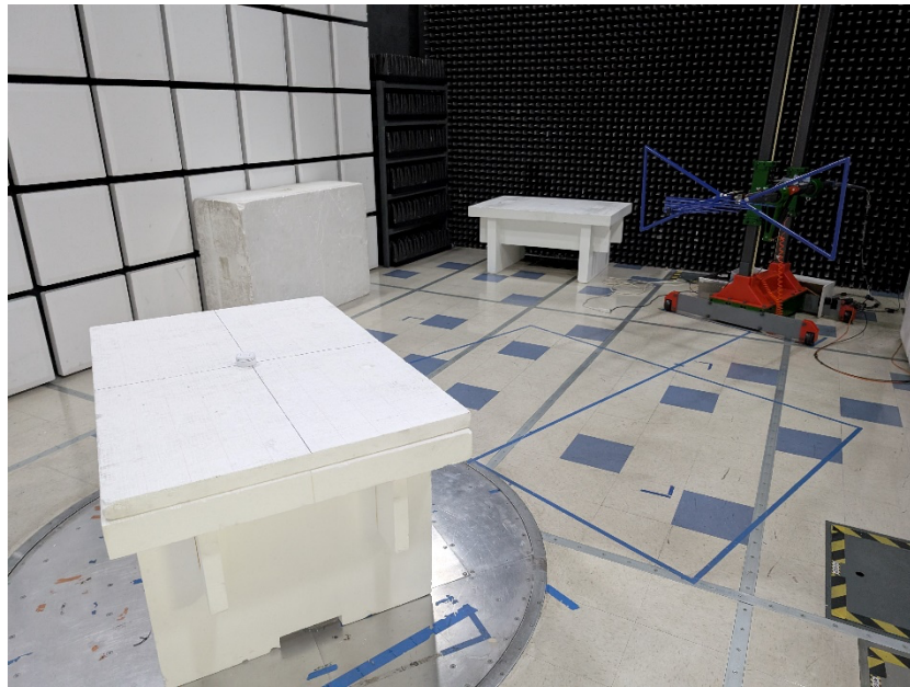
30-1000 MHz Radiated Emission Setup
