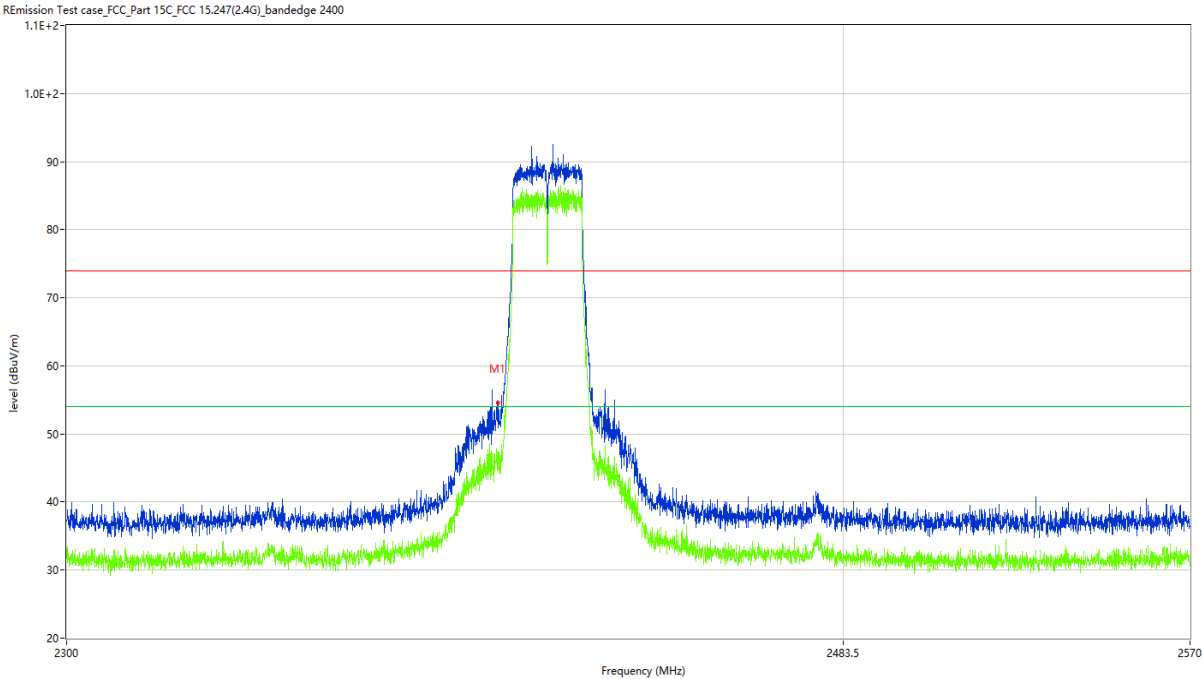
Figure 52: Band Edge (Restricted-band band-edge), 802.11g, 2412MHz Horizontal
