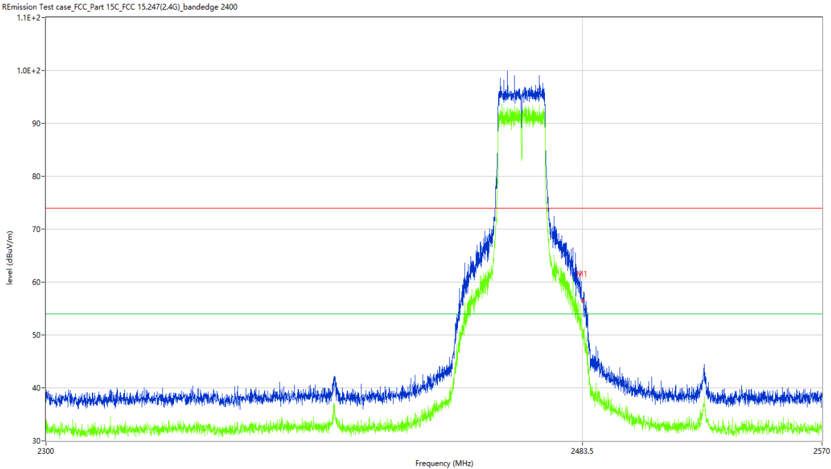
Figure 53: Band Edge (Restricted-band band-edge), 802.11g, 2462MHz Horizontal
