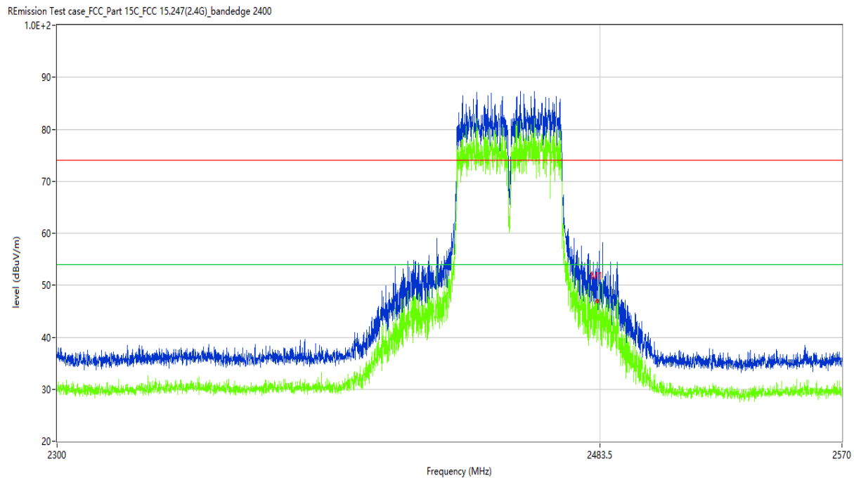
Figure 57: Band Edge (Restricted-band band-edge), 802.11n(HT40), 2452MHz
