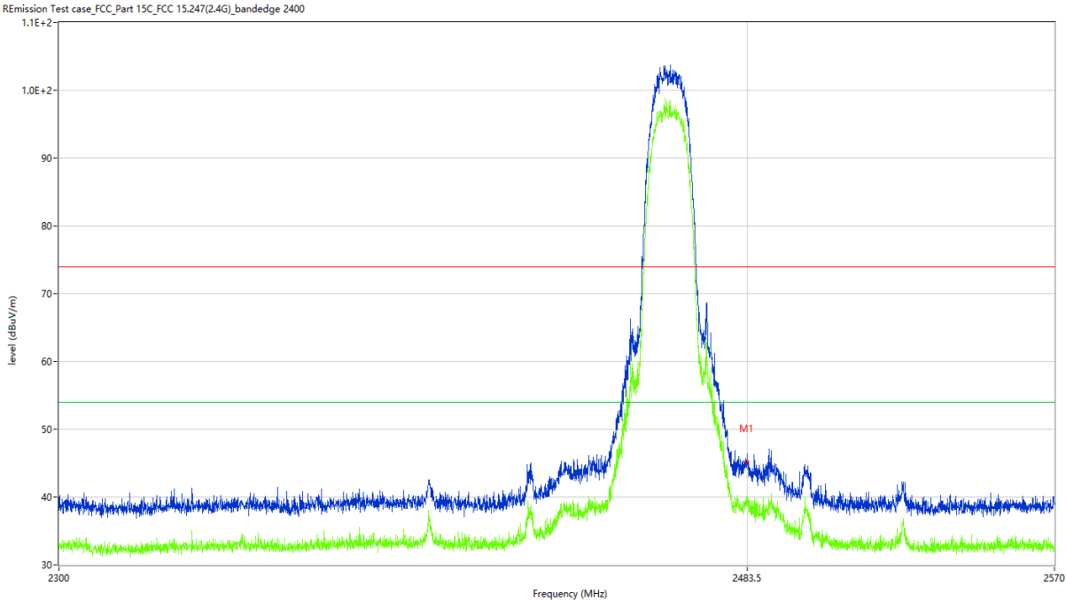
Figure 51: Band Edge (Restricted-band band-edge), 802.11b, 2462MHz Horizontal
