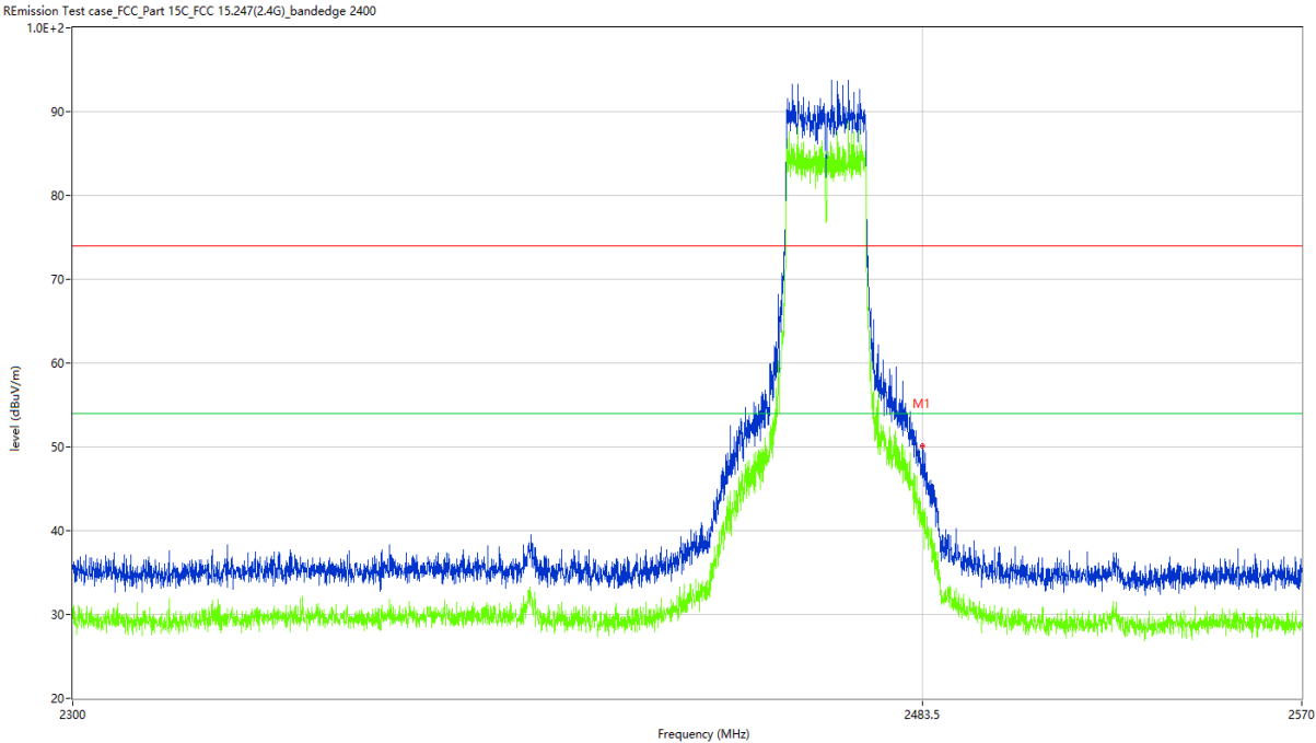
Figure 55: Band Edge (Restricted-band band-edge), 802.11n(HT20), 2462MHz Horizontal
