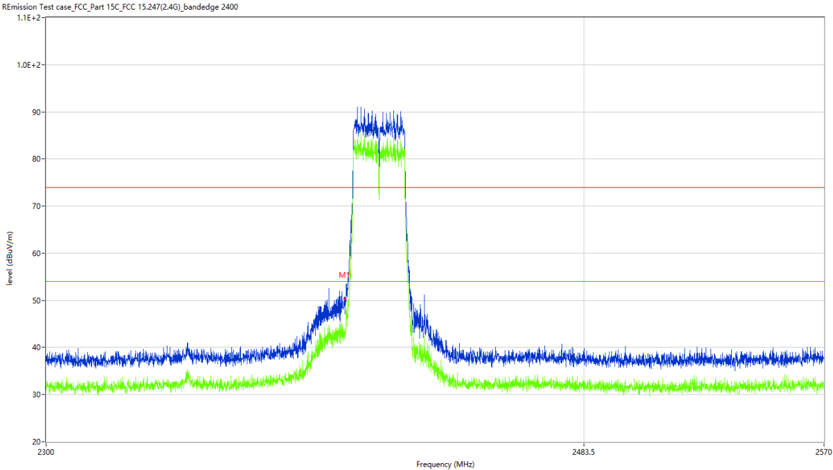
Figure 54: Band Edge (Restricted-band band-edge), 802.11n(HT20), 2412MHz Horizontal
