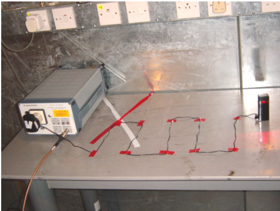
Set-up for Voltage Disturbance in AC mains
