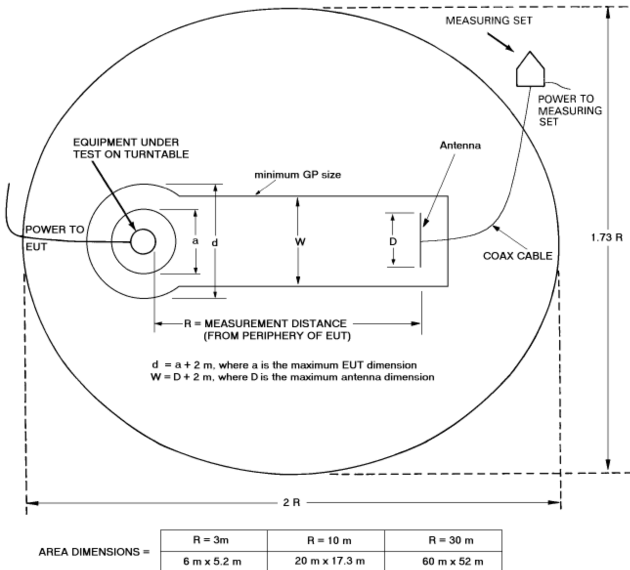
FIGURE 1: RADIATED EMISSIONS 3-METER SEMI -ANECHOIC TEST CHAMBER
