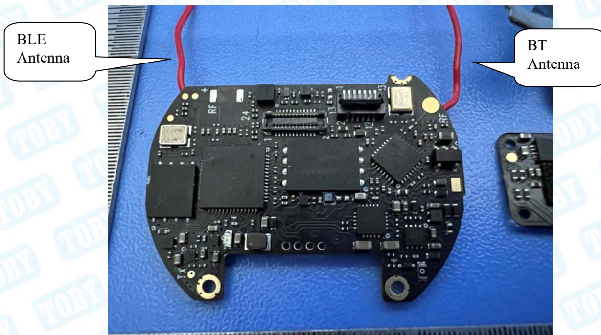
Photo 9 Appearance of PCB
