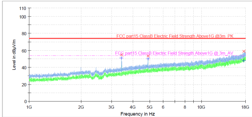
Figure 15: Spectral Diagrams, Radiated Emission, 1GHz-18GHz, Horizontal, BLE 1M 2440MHz
