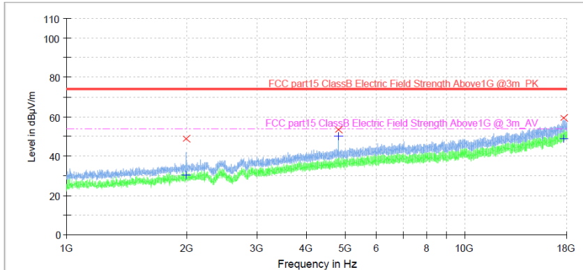
Figure 9: Spectral Diagrams, Radiated Emission, 1GHz-18GHz, Horizontal, BLE 1M 2402MHz
