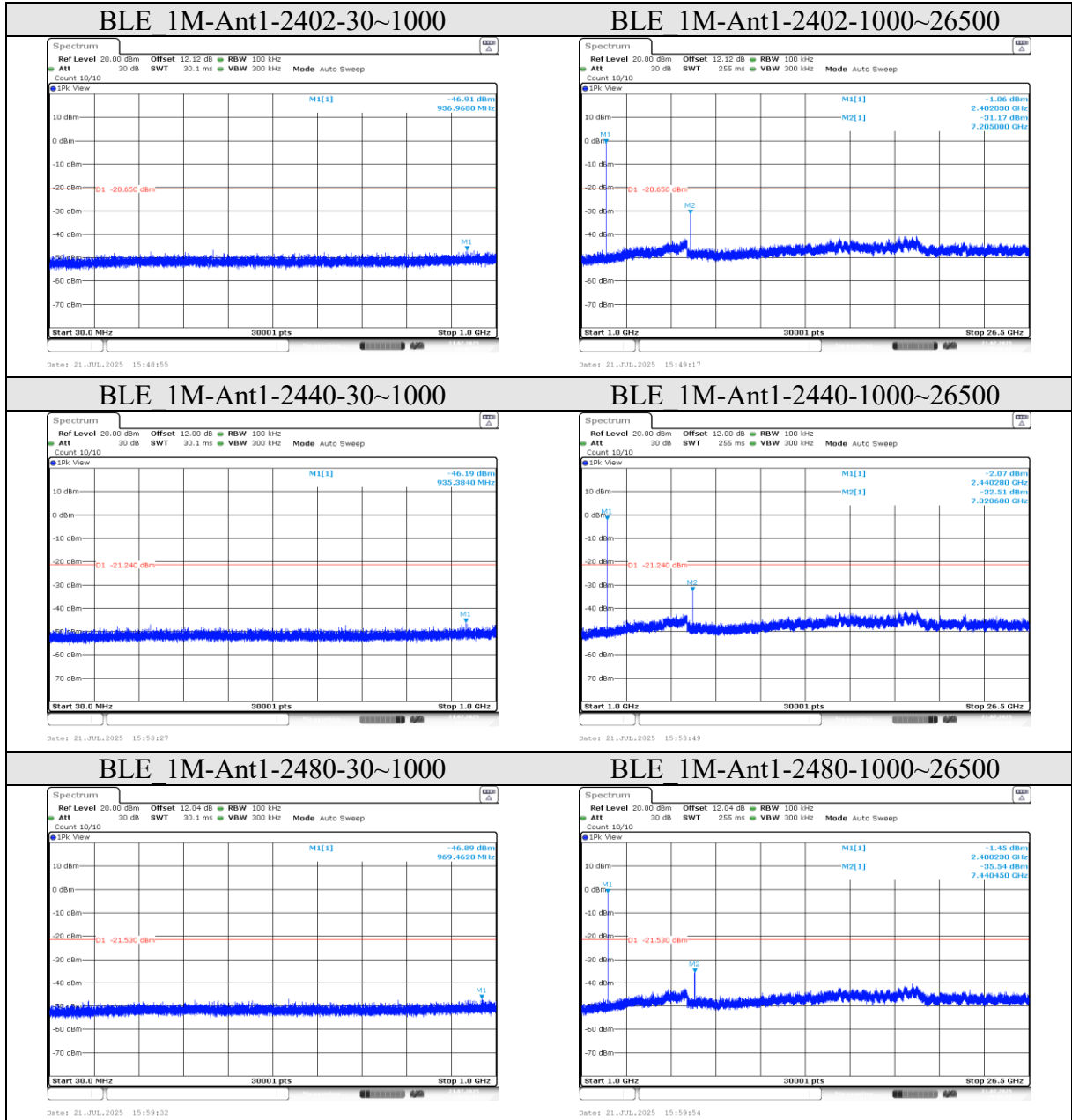
Figure 3: Conducted Spurious Emission
