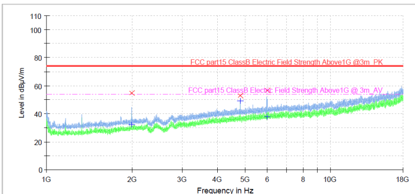
Figure 10: Spectral Diagrams, Radiated Emission, 1GHz-18GHz, Vertical, BLE 1M 2402MHz
