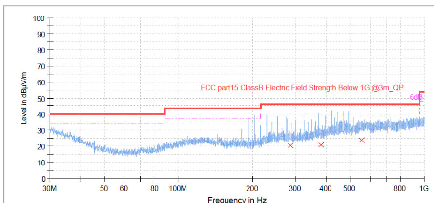
Figure 19: Spectral Diagrams, Radiated Emission, 30MHz-1000MHz, Horizontal, BLE 1M 2480MHz
