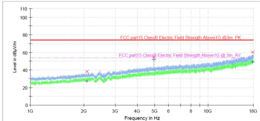
Figure 21: Spectral Diagrams, Radiated Emission, 1GHz-18GHz, Horizontal, BLE 1M 2480MHz
