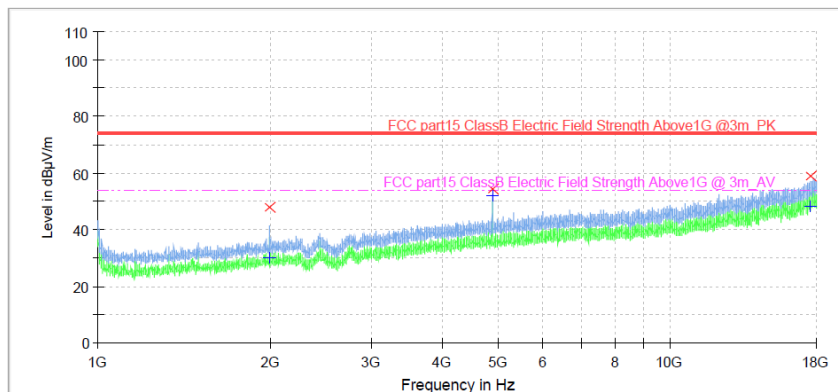
Figure 16: Spectral Diagrams, Radiated Emission, 1GHz-18GHz, Vertical, BLE 1M 2440MHz
