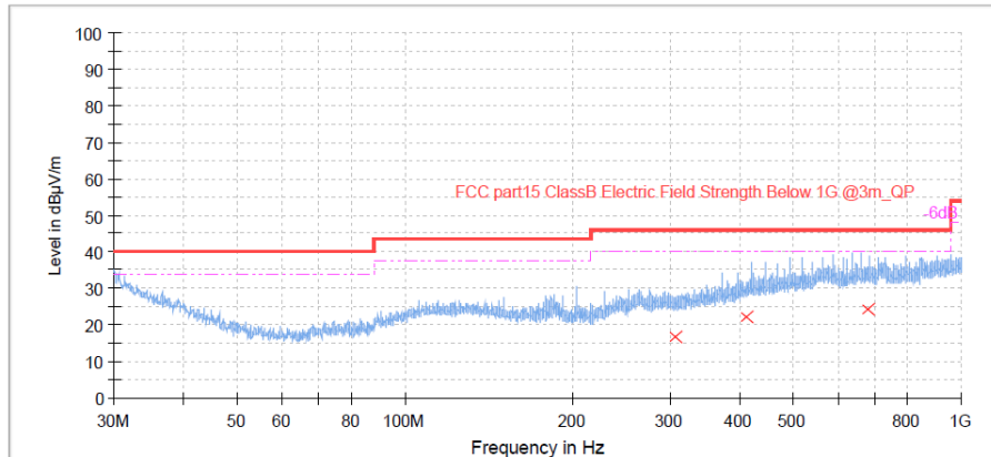
Figure 8: Spectral Diagrams, Radiated Emission, 30MHz-1000MHz, Vertical, BLE 1M 2402MHz
