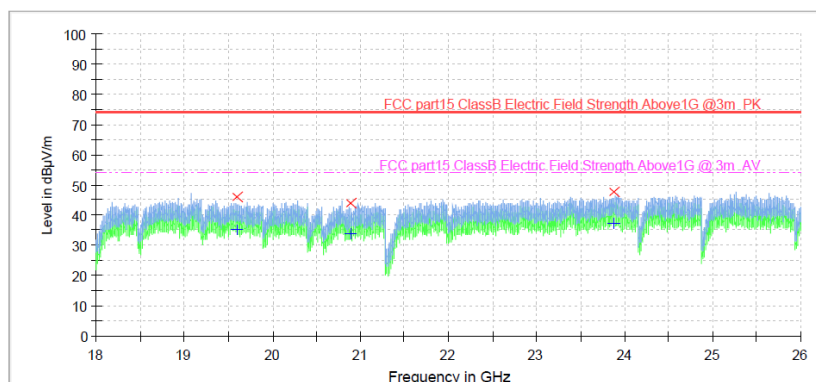
Figure 24: Spectral Diagrams, Radiated Emission, 18GHz-26GHz, Vertical, BLE 1M 2480MHz
