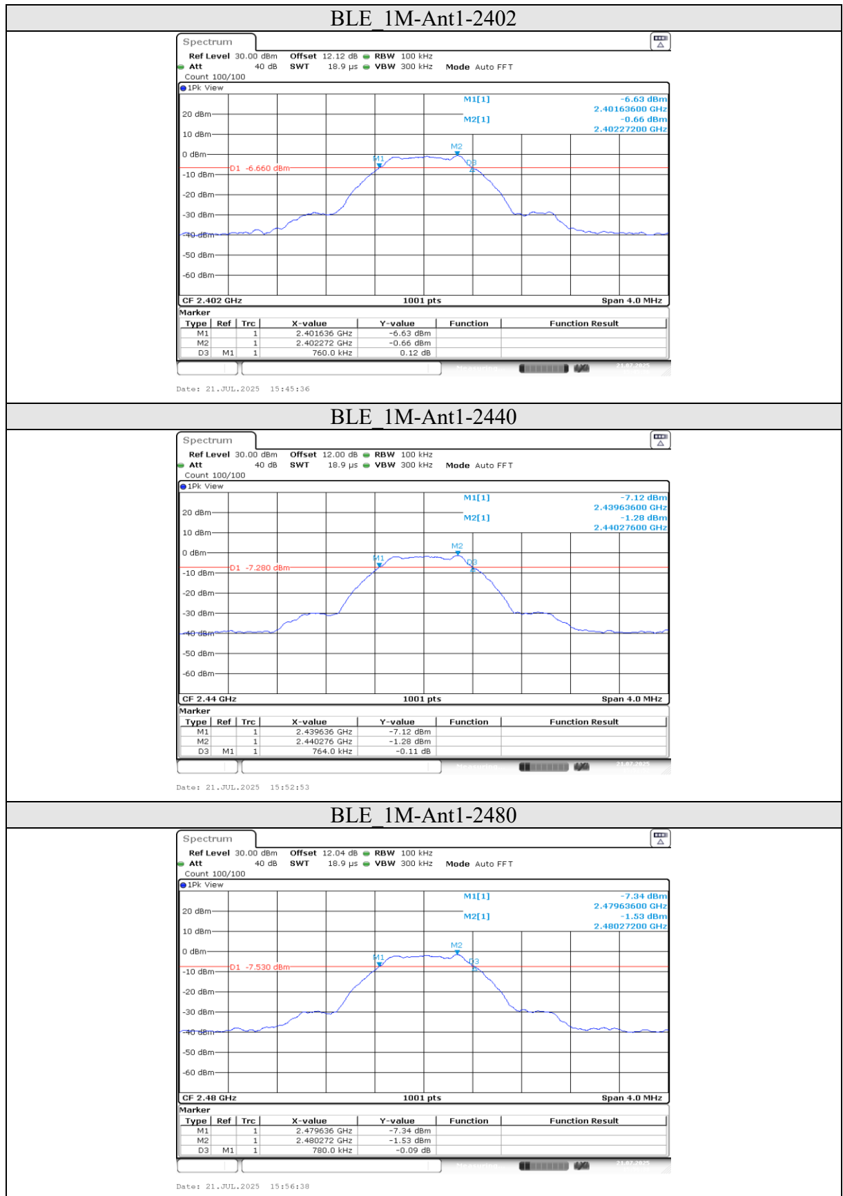
Figure 1: 6dB Bandwidth
