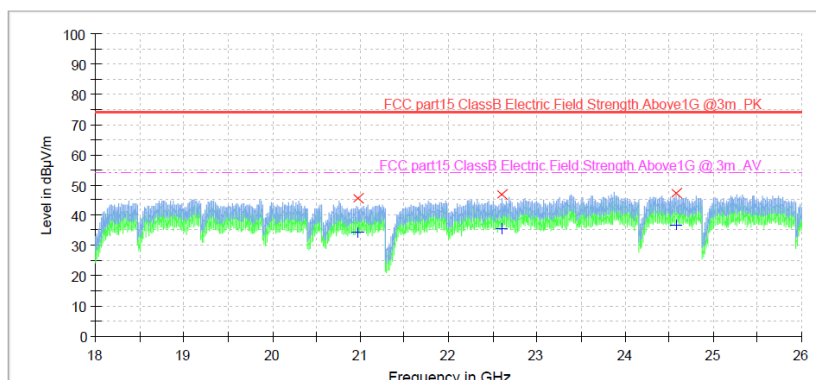
Figure 23: Spectral Diagrams, Radiated Emission, 18GHz-26GHz, Horizontal, BLE 1M 2480MHz
