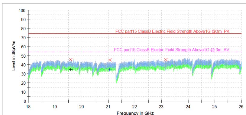
Figure 17: Spectral Diagrams, Radiated Emission, 18GHz-26GHz, Horizontal, BLE 1M 2440MHz
