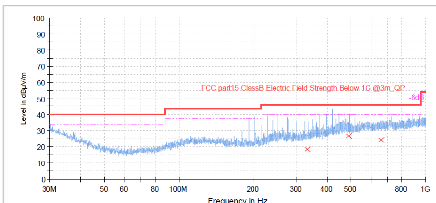
Figure 13: Spectral Diagrams, Radiated Emission, 30MHz-1000MHz, Horizontal, BLE 1M 2440MHz
