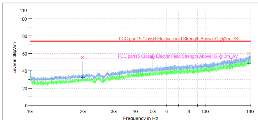
Figure 22: Spectral Diagrams, Radiated Emission, 1GHz-18GHz, Vertical, BLE 1M 2480MHz
