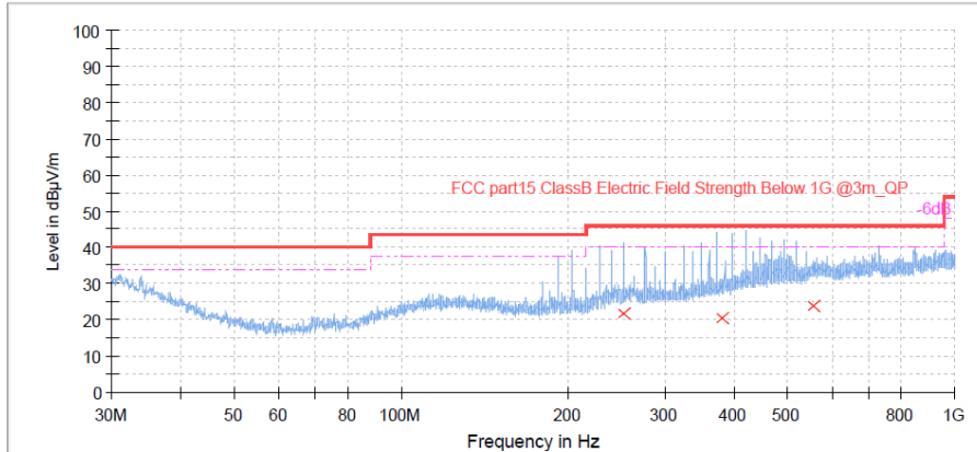
Figure 7: Spectral Diagrams, Radiated Emission, 30MHz-1000MHz, Horizontal, BLE 1M 2402MHz
