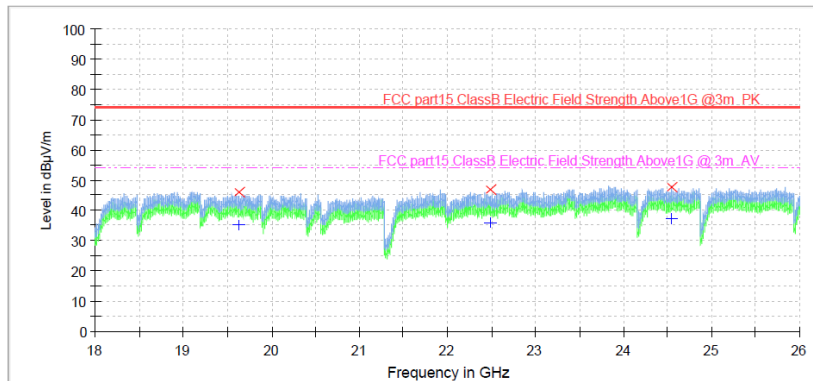
Figure 11: Spectral Diagrams, Radiated Emission, 18GHz-26GHz, Horizontal, BLE 1M 2402MHz
