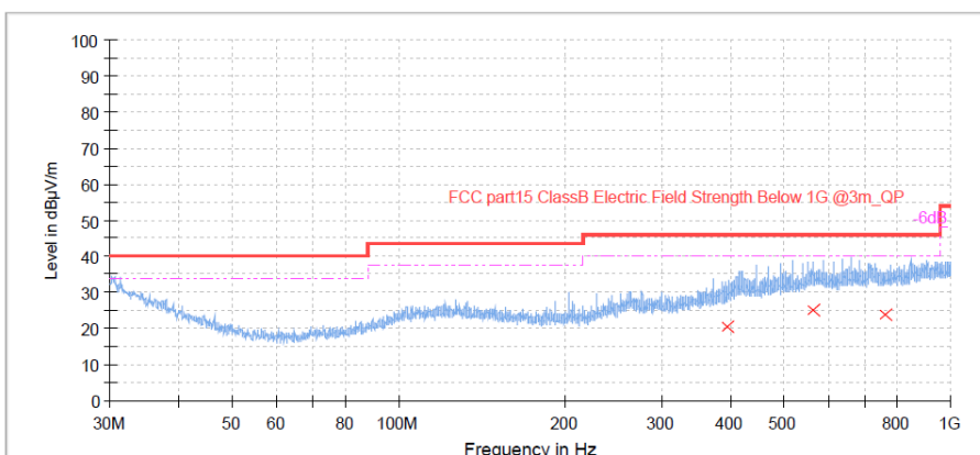
Figure 14: Spectral Diagrams, Radiated Emission, 30MHz-1000MHz, Vertical, BLE 1M 2440MHz
