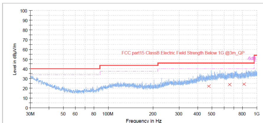
Figure 20: Spectral Diagrams, Radiated Emission, 30MHz-1000MHz, Vertical, BLE 1M 2480MHz
