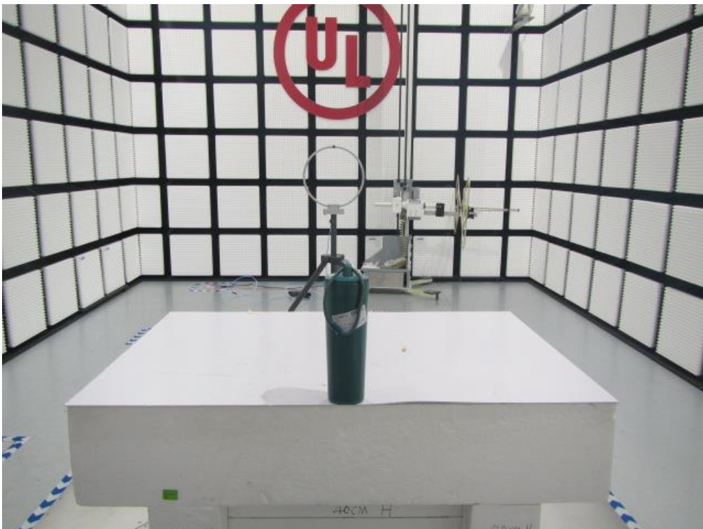
RADIATED DISTURBANCE BELOW 30MHZ MEASUREMENT SETUP
