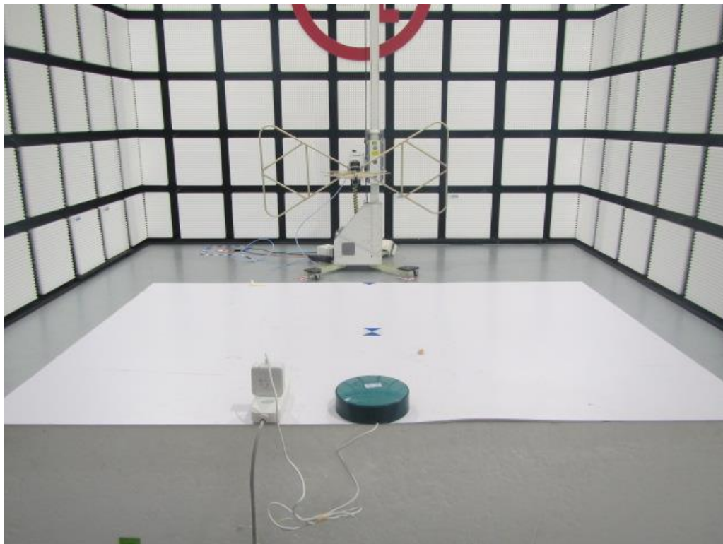
RADIATED DISTURBANCE BELOW 1GHZ MEASUREMENT SETUP FOR SUB 1GHZ
