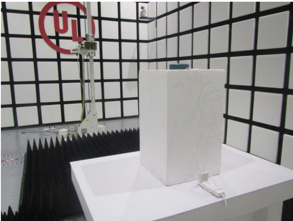
RADIATED RF MEASUREMENT ABOVE 1GHZ SETUP FOR SUB 1GHZ
