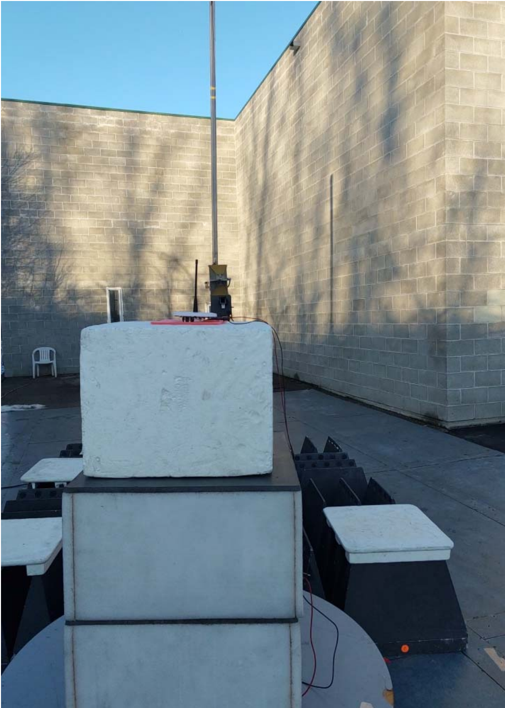
Figure E21.3 – Setup Photo – Radiated Rx, 1 – 5GHz, Antenna A
