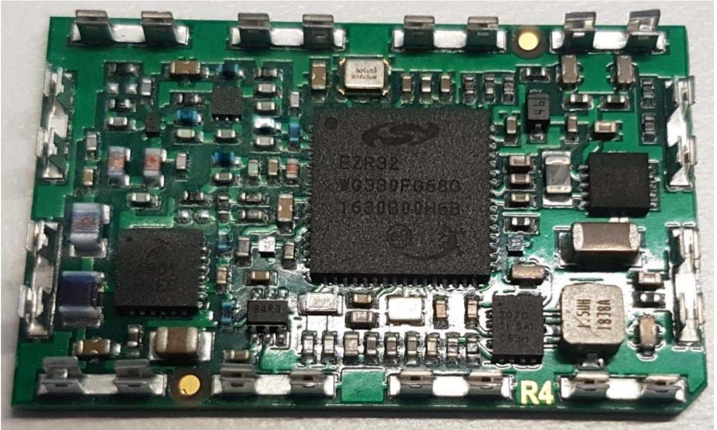
Figure E20.1 – Internal – Shield Removed
