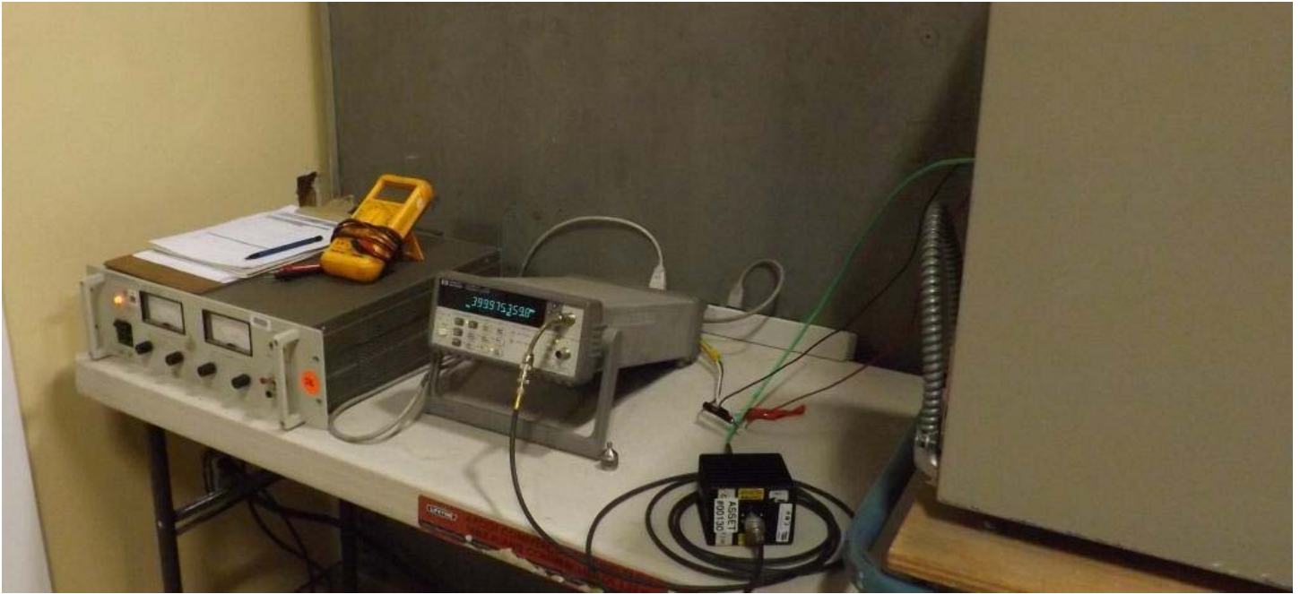
Figure E21.7 – Test Set Up - Frequency Stability
