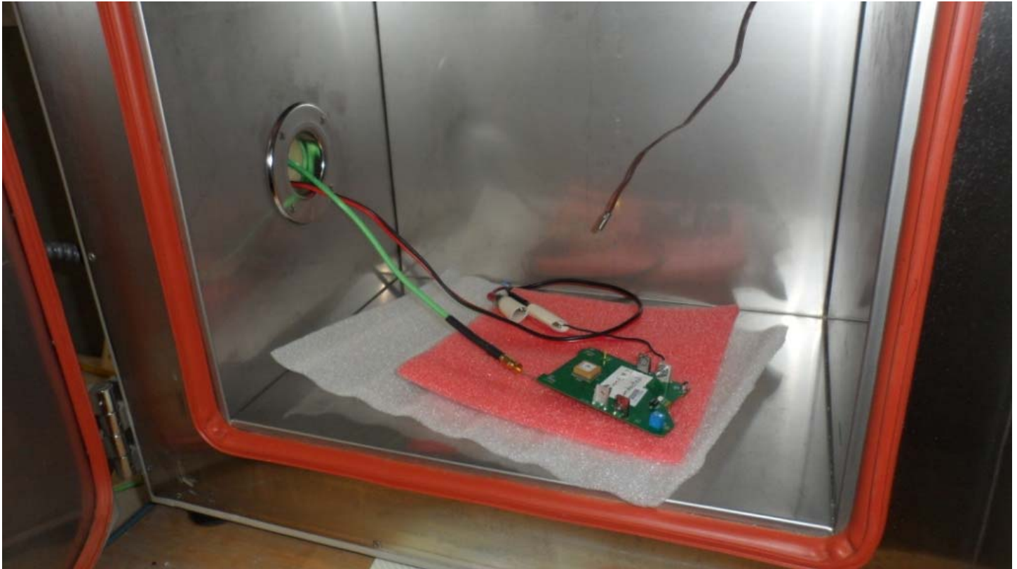
Figure E21.2 – Setup Photo – Frequency Stability Measurements
