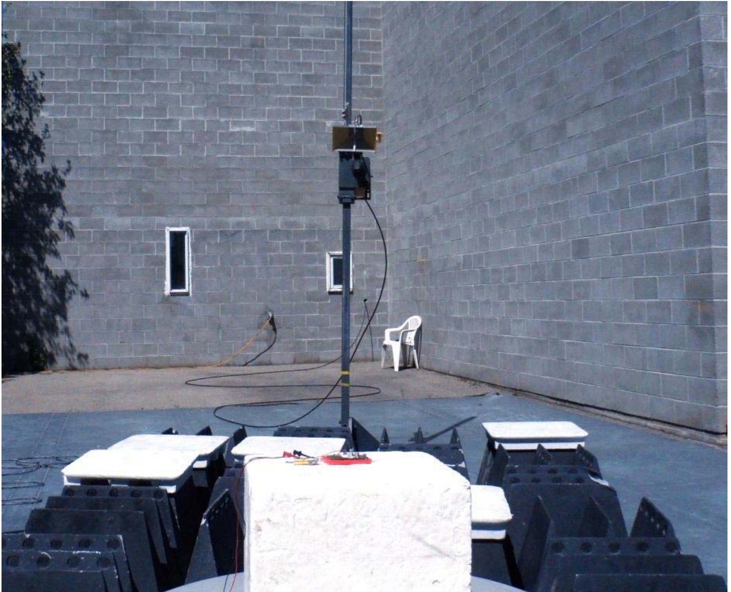
Figure E21.6 – Setup Photo – Radiated Measurements - > 1GHz
