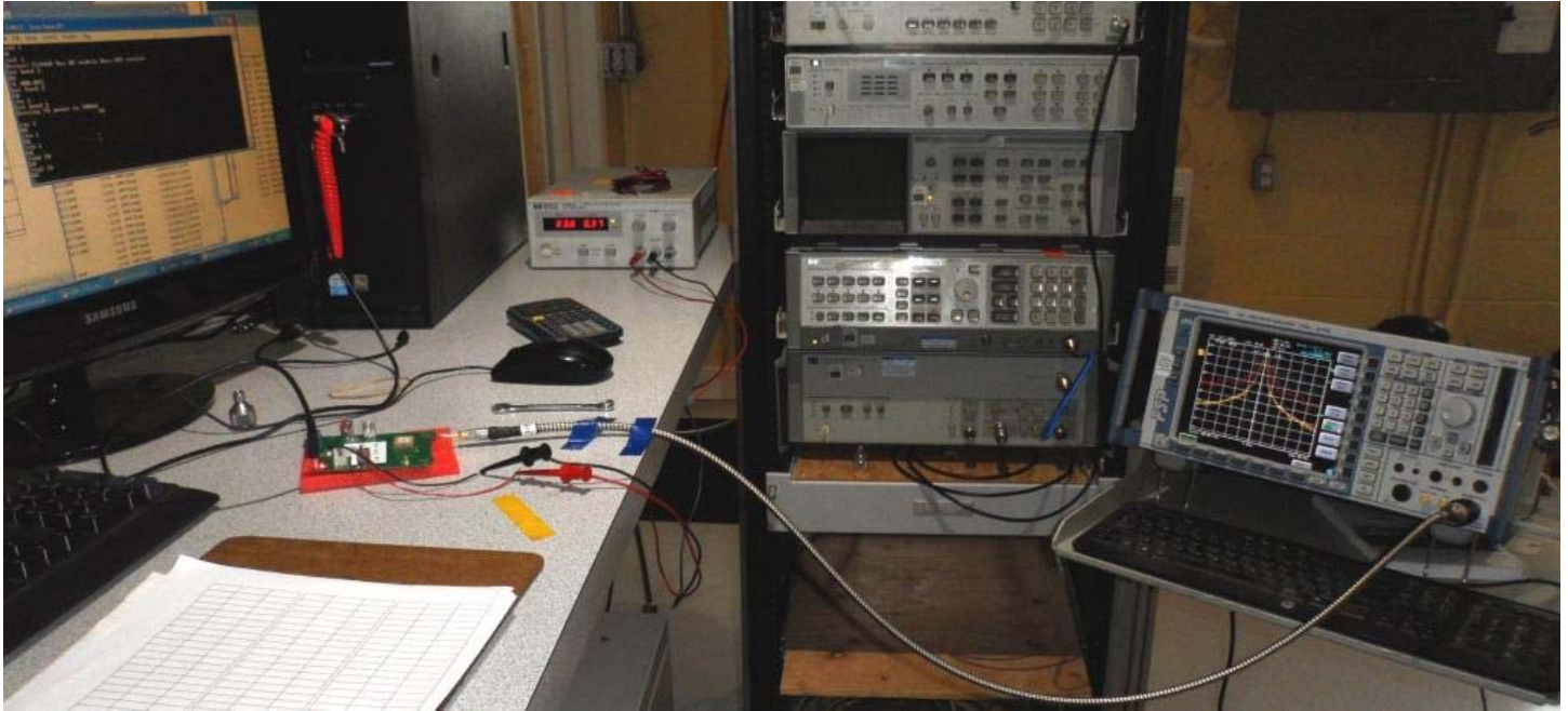
Figure E21.1 – Setup Photo – Conducted Measurements
