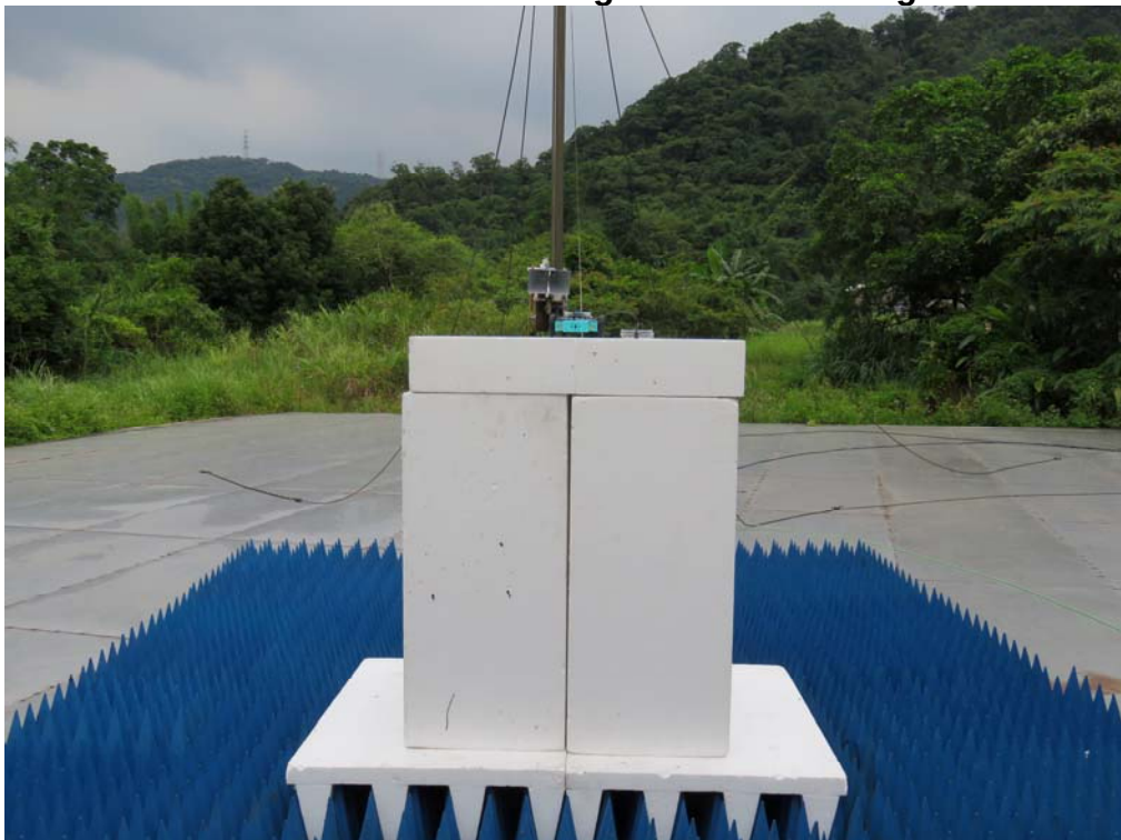
Rear View of The Test Configuration – Working mode
