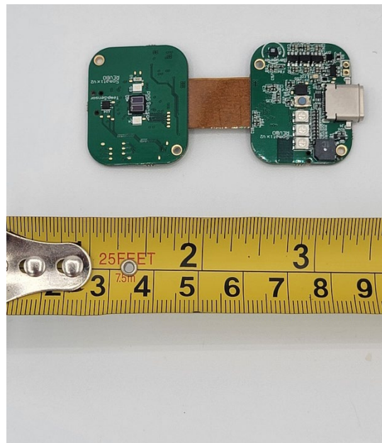
PCB – Bottom view
