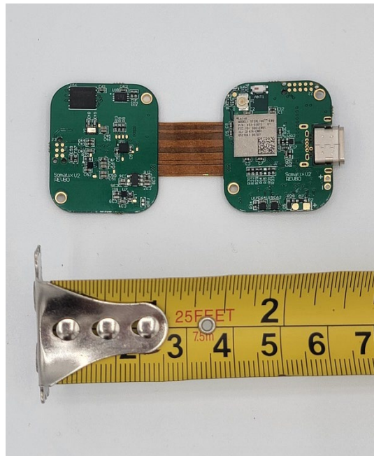
PCB – Bottom view
