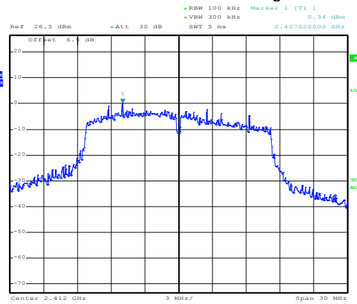
Test mode: 802.11g
