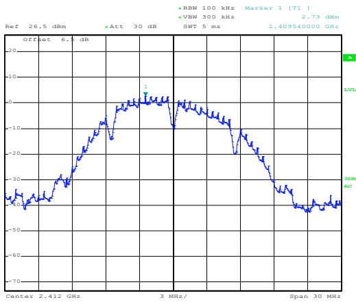
Test mode: 802.11b
